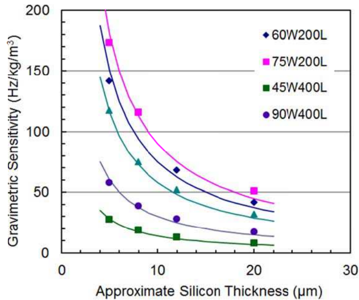
Figure 8: The gravimetric sensitivity of coated cantilevers as a function of the silicon thickness for 200 μm and 400 μm long beams with different widths. The cantilevers are coated with a 2 μm thick polymer film with a density of 840 kg/m 3 . The gravimetric sensitivity of the devices was extracted from modal analyses performed using the finite element software COMSOL. The key in the upper right hand corner gives the size of the cantilever associated with each set of datapoints i.e. 60W200L indicates a 60 μm wide by 200 μm long cantilever.
