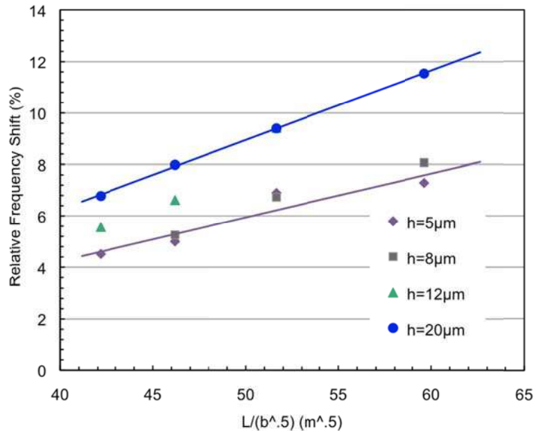
Figure 7: Percentage frequency shift of the first in-plane flexural mode when immersed in water (compared to value in air) as a function of the cantilever length divided by the square root of the cantilever width for cantilevers with a length of 400 μm.
