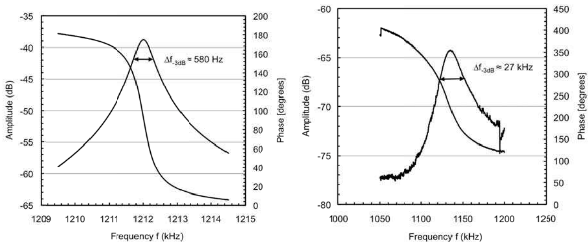
Figure 3: Amplitude and phase transfer characteristic for a 45 \mu\text{m} wide, 200 \mu\text{m} long and 8 \mu\text{m} thick cantilever in air (left) and in water (right).
