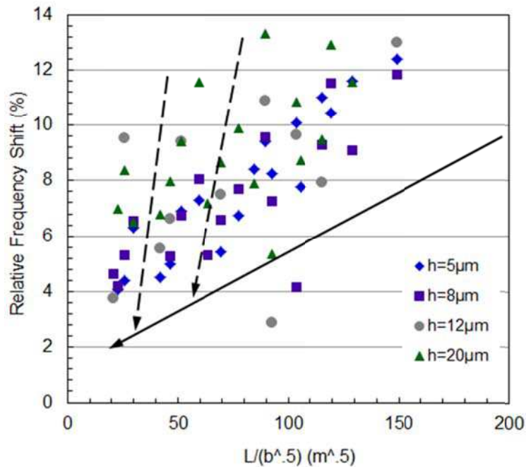
Figure 5: Relative frequency shift of the first in-plane flexural mode when immersed in water (compared to its value in air) as a function of cantilever length divided by the square root of the cantilever width for cantilevers with silicon thicknesses of 5, 8, 12 and 20 μm. The solid arrow indicates the overall trend of a reduced frequency shift with decreasing L/b^{1/2} ratio, i.e. increasing resonance frequency. The dashed arrows show the trend for a given cantilever length (in this case 200 and 400 μm), where the frequency shift rapidly decreases with increasing beam width (see also Fig. 6).
