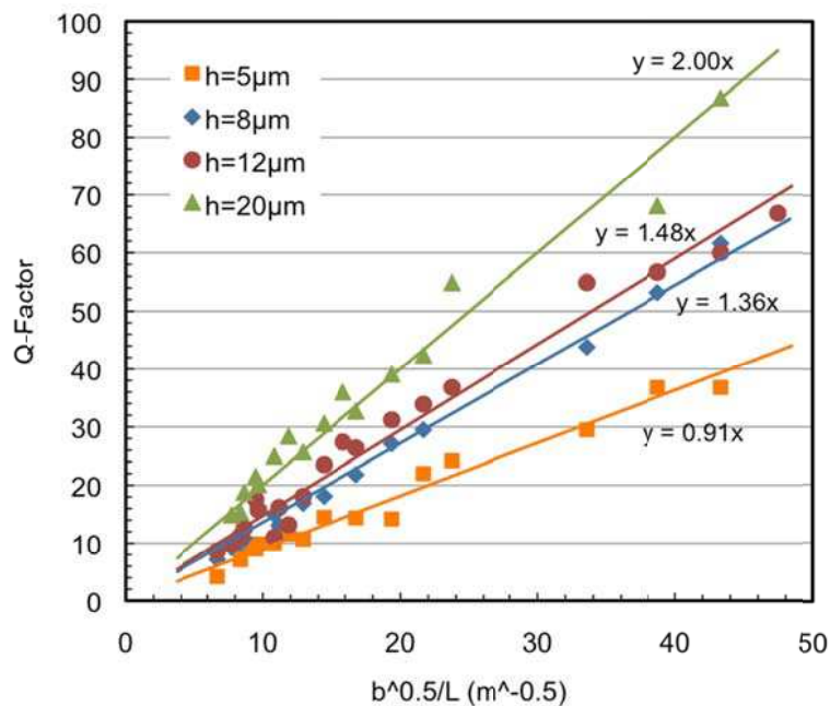
Figure 4: Q-factor of in-plane bending mode for cantilevers with 5, 8, 12 and 20 \mu\text{m} silicon thickness in water as a function of b^{1/2}/L (square root of beam width divided by length), which is – to first order – proportional to the square root of the resonance frequency. (Lines are linear fits of the data for a given device thickness.)
