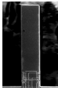
Figure 1: SEM image of a fabricated 45 \mu\text{m} wide and 200 \mu\text{m} long cantilever. The Wheatstone bridge and excitation resistors are visible at the base of the device.
