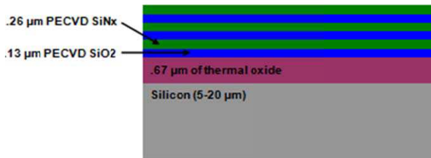
Figure 2: Cross section of the tested cantilevers. Note that thickness values given in the text of the paper are those of the silicon layer only and do not include the thermal oxide or PECVD passivation layers.
