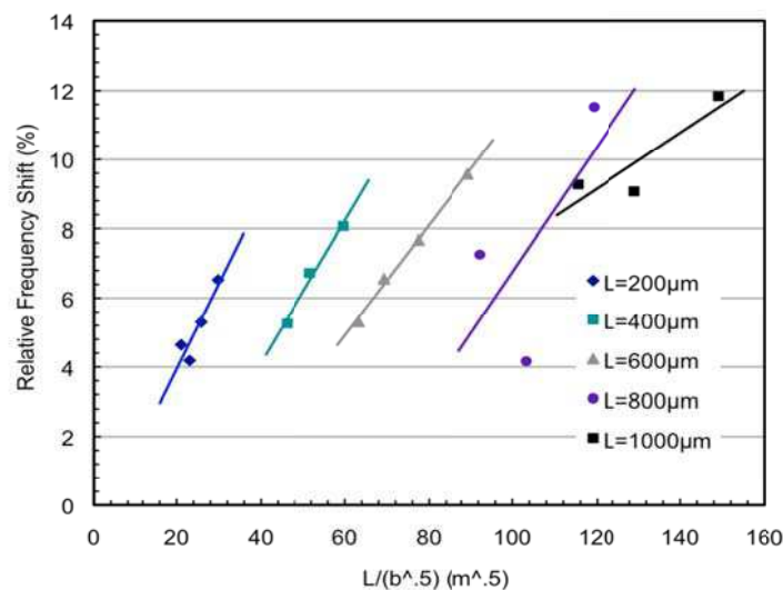
Figure 6: Percentage frequency shift of the first in-plane flexural mode when immersed in water (compared to value in air) as a function of the cantilever length divided by the square root of the
