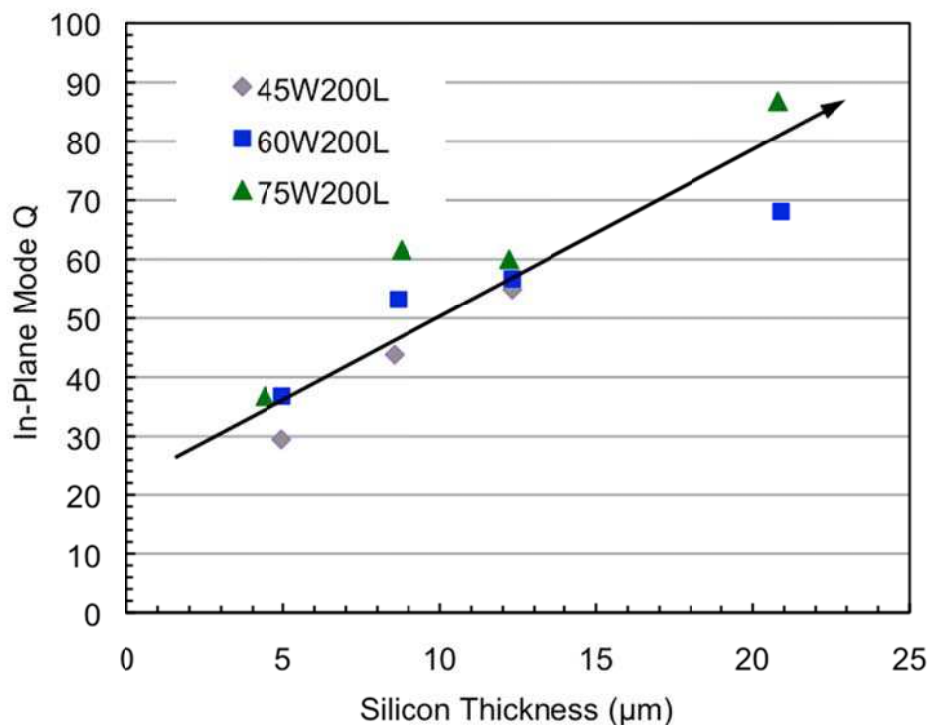
Figure 9: Quality factor as a function of silicon thickness for 200 \mu\text{m} long cantilevers operated in water. The key in the upper left hand corner gives the size of the cantilever associated with each set of points i.e. 45W200L indicates a 45 \mu\text{m} wide by 200 \mu\text{m} long cantilever.
