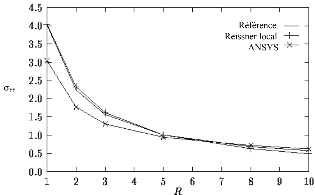
Fig.4- \sigma_{yy} au point E \sigma_{yy} at point E
