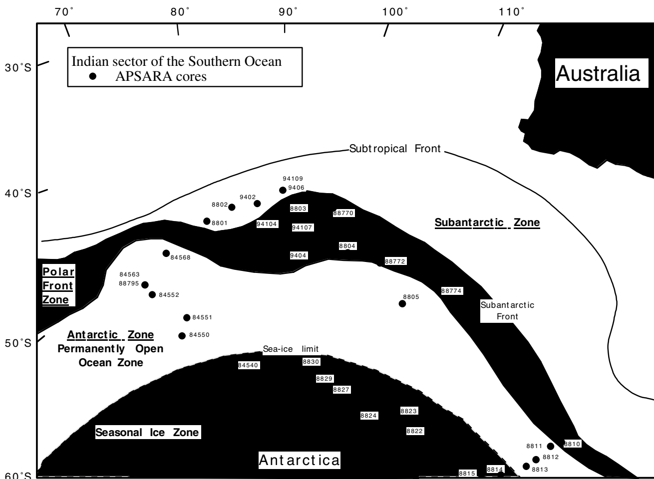
Figure 1b. Map showing the location of the sediment sampling sites in the Indian sector of the Southern Ocean. The present-day position of the oceanographic fronts are from Bareille [1991] and Bareille et al. [1991] . The dashed area limits the oceanic zone covered by ice. The dark shaded area highlights the position of the Polar Front Zone.
