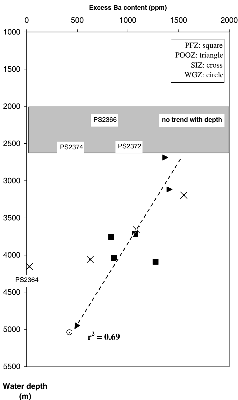
Figure 4a. Excess Ba content reported as a function of the water column depth for the Atlantic sector of the Southern Ocean. Data are from Table 2. For the samples deeper than 2500 m water depth the Baxs content decreases with increasing water depth. This may reflect a higher dissolution of barite crystals in progressively undersaturated waters.
