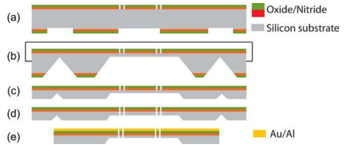
Fig. 9. Fabrication process chain for the tilt mirror. Process description. (a) Defining the mirror structures on the passivation layer on both sides of the substrate. (b) KOH etch from the backside of the Si substrate. (c) Wafer thinning (optional) and chip separation. (d) ICP etch from the front side of the mirror. (e) Deposition of a gold layer to improve the reflectivity of the mirror.
