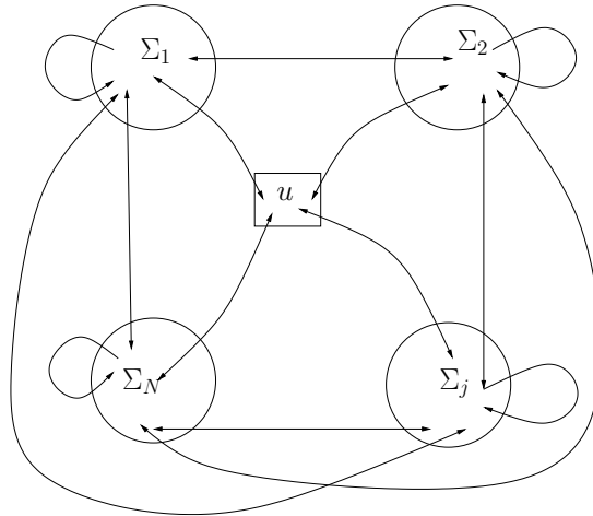
FIGURE 1. Our system
