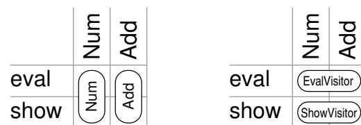
(a) Data decomposition (program P_{data} ).
