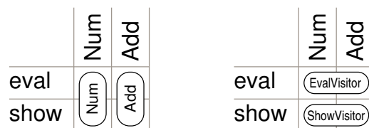
(a) Data decomposition (program P_{data} ).
