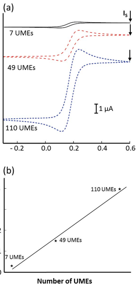
Fig. 4 (a) Cyclic voltammograms (scan rate: 50 mV s^{-1} ) at 7, 49 and 110 UMEs in aqueous solution containing K_4[Fe(CN)_6] (5 mM); (b) linear variation of steady current ( I_s ) vs. number of short-circuited UMEs.
