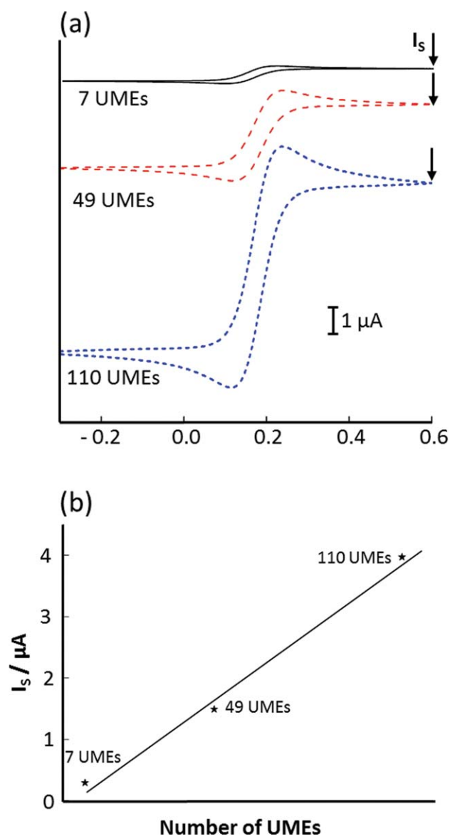
Fig. 4 (a) Cyclic voltammograms (scan rate: 50 mV s^{-1} ) at 7, 49 and 110 UMEs in aqueous solution containing K_4[Fe(CN)_6] (5 mM); (b) linear variation of steady current ( I_s ) vs. number of short-circuited UMEs.
