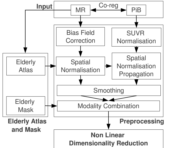
Figure 1: Overview of the algorithmic pipeline
