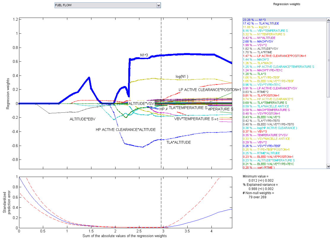
Figure 4: The result of the LARS/LASSO algorithm when selecting inputs for fuel flow regression. The upper graph shows the coefficients \lambda when the energy constraint C increases. The lower graph gives the generalization error obtained by cross-validation. The selected solution is marked by a vertical dashed line. On the right: the sorted (selected) inputs with their relative weights.
