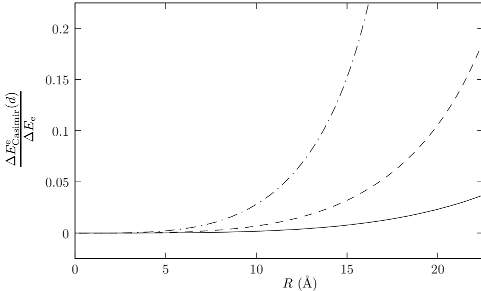
Figure 1: Modification of the Lamb shift in spherical InAs microcrystals for d = 1\mu\text{m} (—), 0.5\mu\text{m} (---) or 0.25\mu\text{m} (-·-).
