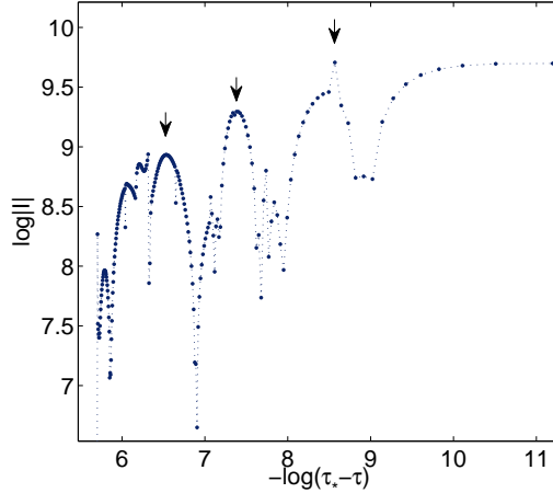
Figure 6. The variation of I obtained in a 4-level AMR simulations initialized by \sigma_r = 0.9 , \sigma_z = 1.3 , and a/a_* \simeq 0.99997 . The variation of \log |I| on each oscillation (marked by arrows) is nearly equal to the temporal period of the echos, \Delta_r \simeq \Delta_\tau \simeq 1.1 .
