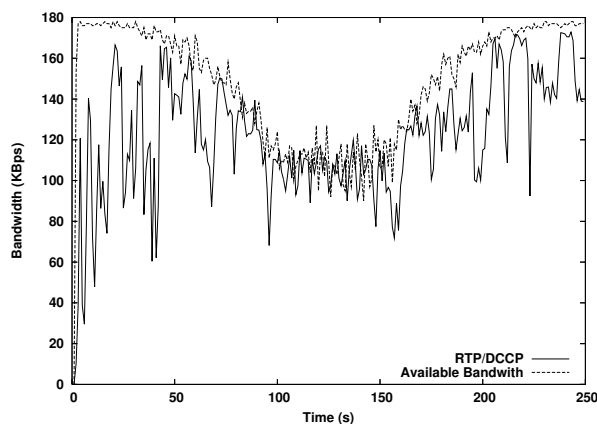
Figure 5: Throughput comparison.
