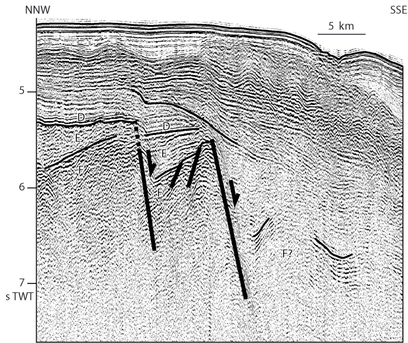
Figure 9 : Seismic line GUYAPLAC 22-23, located in Figures 1 and 5. Faults are not directly observed in the acoustic basement, but drawn from offsets and tilts of the overlying seismic reflectors. Vertical exaggeration 13 in water.
