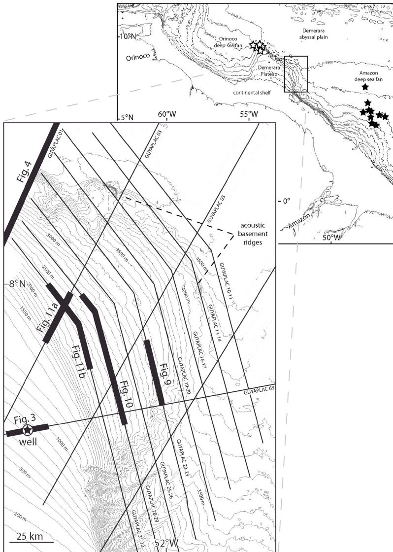
Figure 1 : Location of GUYAPLAC seismic lines in the eastern Demerara plateau. Bathymetry from GUYAPLAC cruise and SHOM data (equidistance 100 m). The upper box locates the Demerara plateau and the Orinoco and Amazon deep sea fans on the northern margin of South America. Stars indicate wells: open stars are sites from Leg ODP 207 (Shipboard Scientific Party, 2004), black stars are Leg ODP 155 sites (Flood et al., 1995), the circled black star locates industrial well G2 described by Gouyet (1988).
