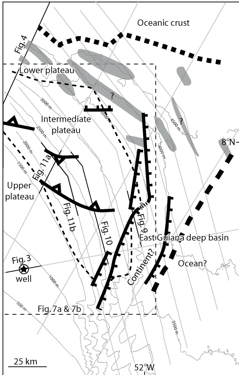
Figure 5 : Structural map of the eastern Demerara plateau. GUYAPLAC seismic lines and bathymetry (equidistance 500 m) are reported. The confidence in the interpolations between seismic lines depends obviously on their wide spacing. The thick dotted lines tentatively limit the oceanic crust northward and eastward from their depths and geophysical properties (see Figure 8 and text for comments). The thin dotted lines limit the various structural parts of the Demerara plateau. The bathymetric plateau extends down to 4500 m northward, and 4000 m eastward, but the basement characters are similar in the lower plateau and eastward below the abyssal plain. Faults are not directly observed in the acoustic basement, but drawn from offsets and tilts of the overlying seismic reflectors. The map traces of the faults correspond to their intersection with the top of the acoustic basement. Most of fault slip occurred before Unit D deposition. At the given map scale, anticline axes are too close to the thrusts to be shown. They are parallel to the thrusts and located on their hanging wall (Figure 6).
