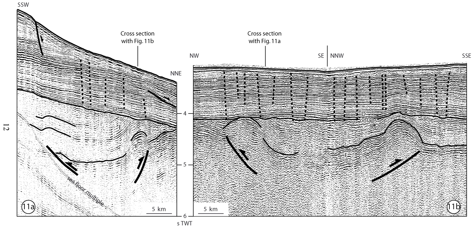
Figure 11 : Seismic lines GUYAPLAC 3 (11a) and 31-32 (11b), located in Figures 1 and 5. Faults are not directly observed in the acoustic basement, but drawn from offsets and tilts of the overlying seismic reflectors. Vertical exaggeration 13 in water.
