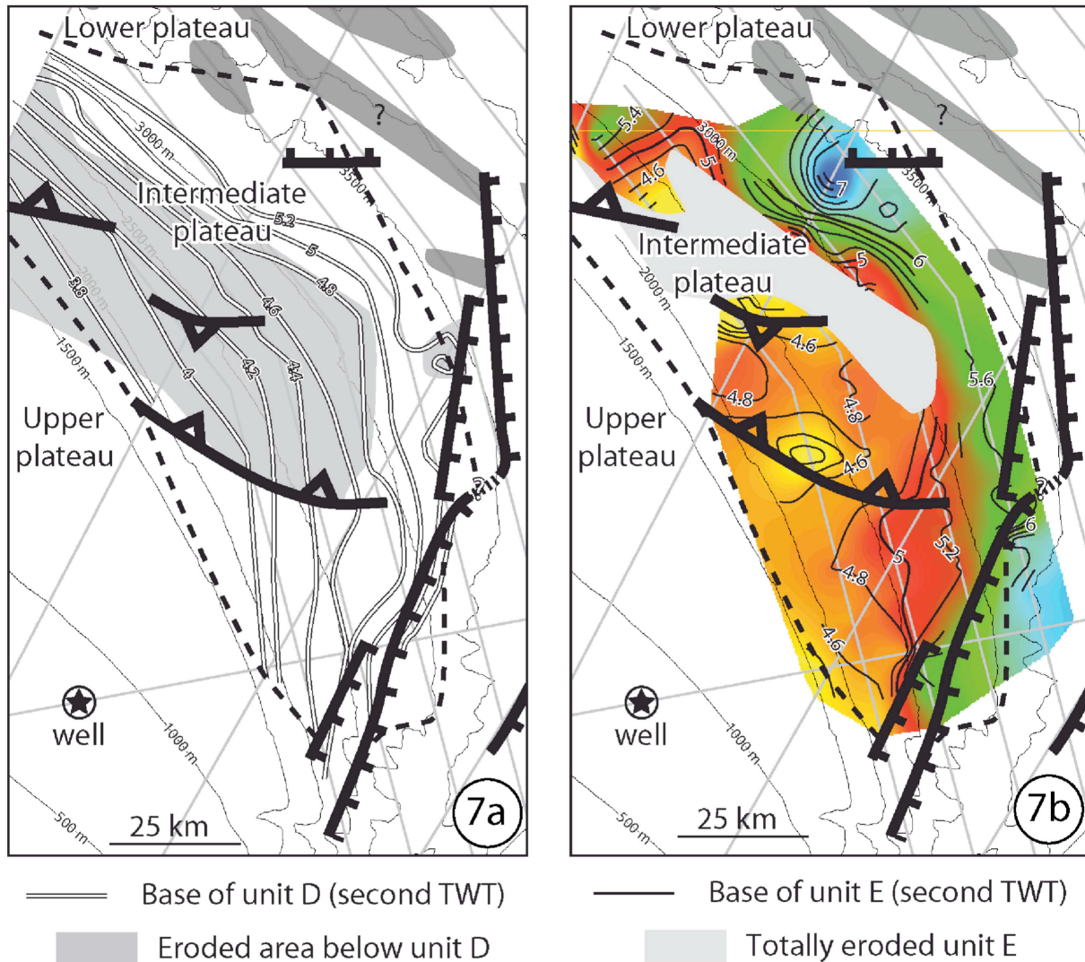
Figure 7 : Depths of the base of unit D (7a) and E (7b) in the intermediate plateau. Structures and bathymetry as in Figure 5. Due to limited seismic penetration, the base of unit E cannot be observed in the deepest parts, and the color interpolation is only weakly constrained.
