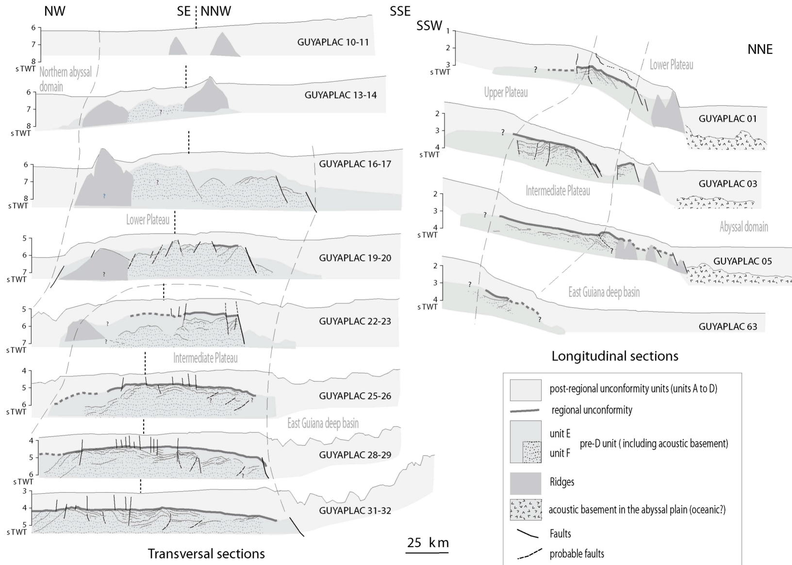
Figure 6 : Line drawings of GUYAPLAC seismic sections, located in Figure 1. The vertical dotted bar indicate change of line strike on transversal sections. Same vertical and horizontal scale for all sections. Vertical exaggeration 13 in water.
