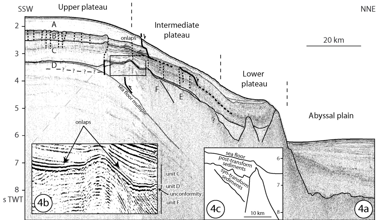
Figure 4 : Seismic line GUYAPLAC 01 (4a, with a local zoom : 4b), located in Figures 1 and 5 (the southwesternmost part of the line extends out of the western edge of Figures 1 and 5). 4c : for comparison, line drawing (same scale as Figure 4a) of a seismic section across the transform margin off Côte d'Ivoire (modified from Basile et al., 1996). A to F are seismic units (see text for details). Thick lines are faults, dotted thick lines are polygonal fault network. Faults are not directly observed in the acoustic basement, but drawn from offsets and tilts of the overlying seismic reflectors. Depth in second double way (sdw). Vertical exaggeration 13 in water.
