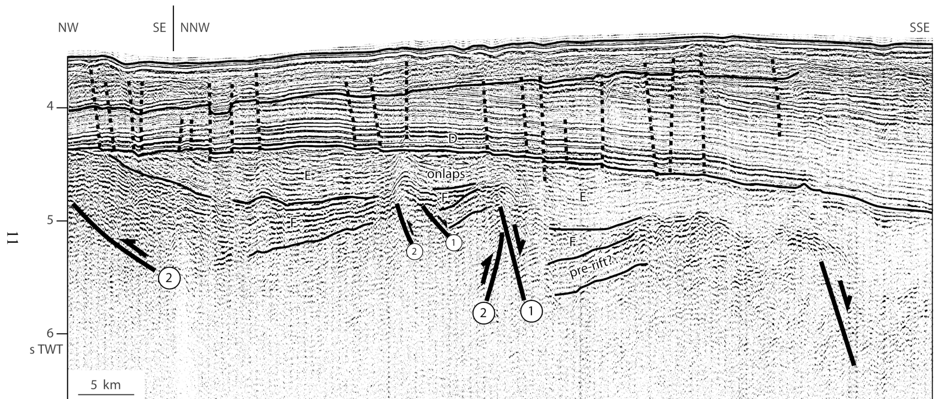
Figure 10 : Seismic line GUYAPLAC 28-29, located in Figures 1 and 5. The circled numbers refer to the first and second stage of deformations, respectively. 1 : normal faults coeval with seismic unit F. 2 : reverse faults reactivating the same structures, coeval with the upper seismic unit E, and older than unit D. Faults are not directly observed in the acoustic basement, but drawn from offsets and tilts of the overlying seismic reflectors. Dotted thick lines indicate faults with polygonal network. Vertical exaggeration 13 in water.
