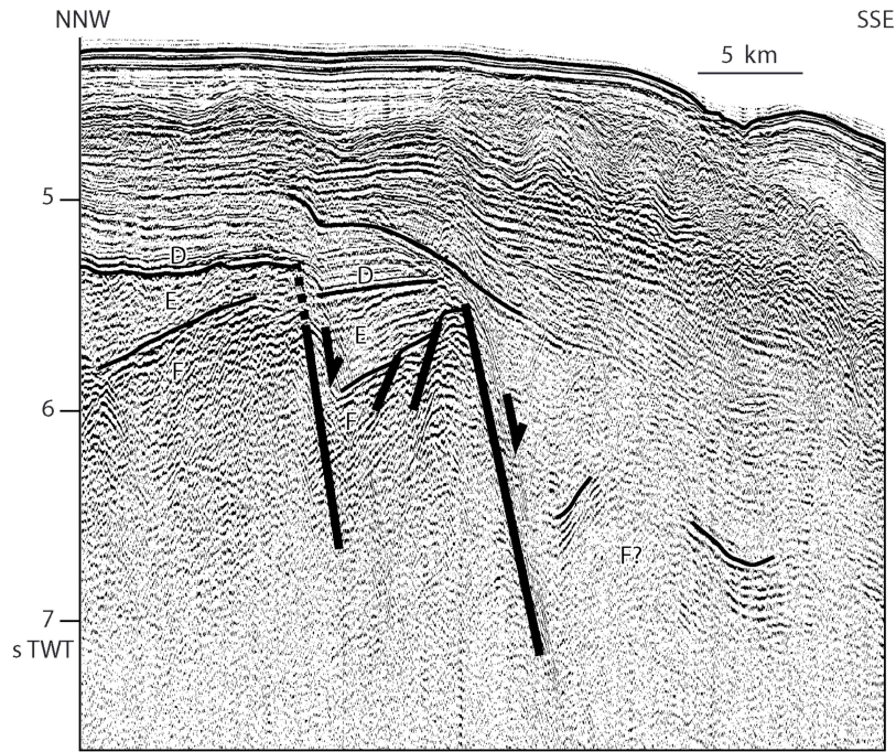
Figure 9 : Seismic line GUYAPLAC 22-23, located in Figures 1 and 5. Faults are not directly observed in the acoustic basement, but drawn from offsets and tilts of the overlying seismic reflectors. Vertical exaggeration 13 in water.
