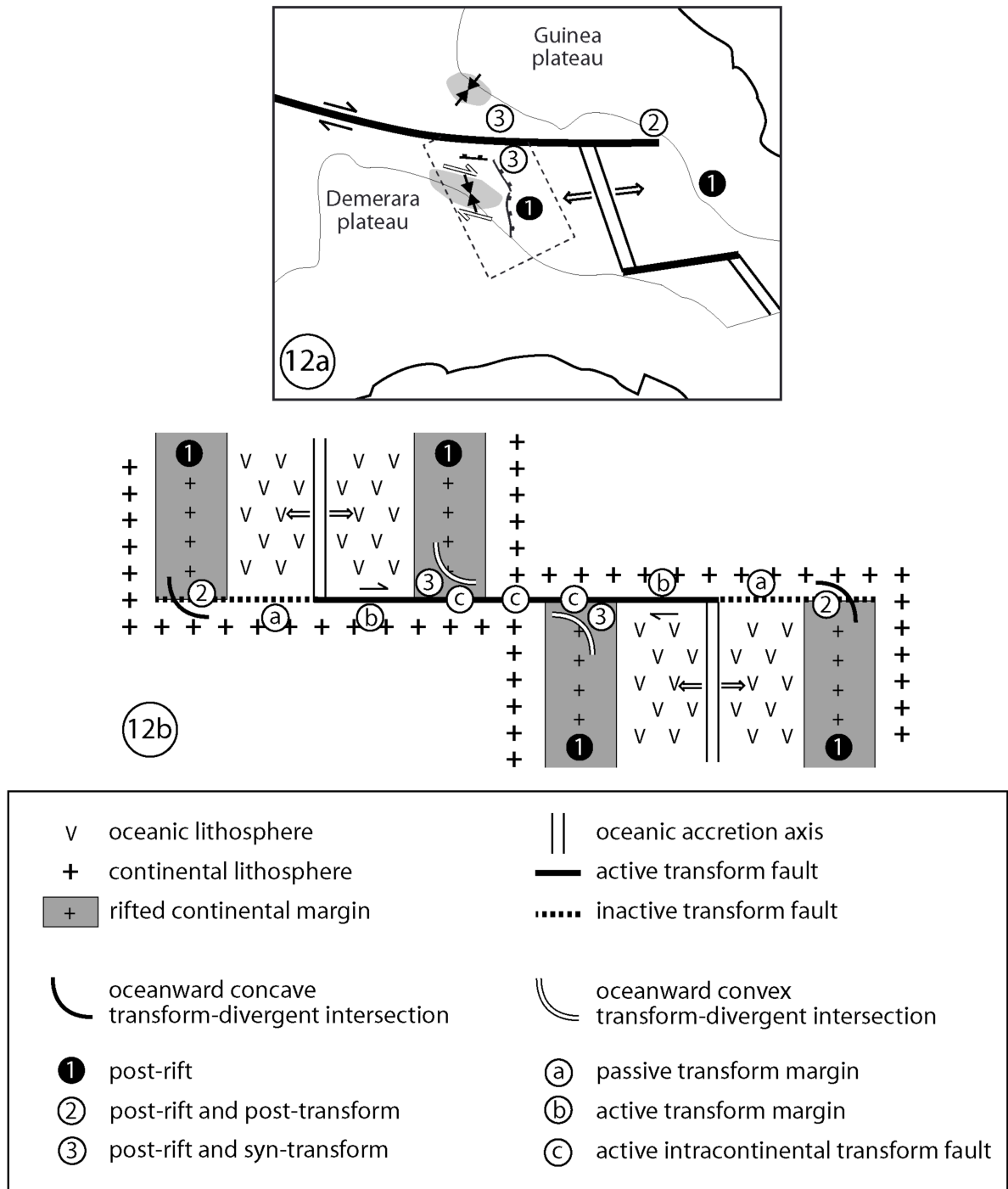
Figure 12 : 12a : Reconstruction of the Demerara and Guinea conjugated margins in their Late Albian (105 Ma) position, with Africa supposed fixed (modified from Basile et al. (2005) and Campan (1995)). The present day coastline and 2 km isobath are drawn. The dotted box indicates the studied area (Figure 5). Post rift shortening occurred in the shaded area, and the black arrows indicate shortening directions. Deformations in the Guinea plateau from Benkhelil et al. (1995). 12b : Asymmetry and diachronism along transform margins and at transform-divergent margins intersections. Concave/convex terminology according to P. De Clarens (personal communication).
