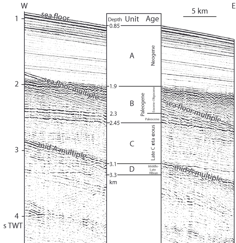
Figure 3 : Seismic units (A to D) from seismic line GUYAPLAC 63, and stratigraphy and approximate depths from well G2 (Gouyet, 1988). The seismic line is located in Figures 1 and 5. Depth in second double way (sdw). Vertical exaggeration 13 in water.
