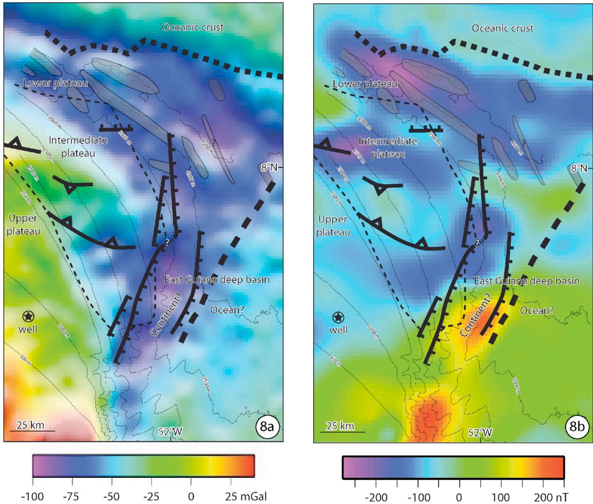
Figure 8 : Geophysical maps of the studied area. Same area and structural features as for Figure 5. 8a : Free air gravity anomaly from satellite altimetry (Sandwell and Smith, 2009). 8b : Magnetic anomaly from gridded GUYAPLAC data.
