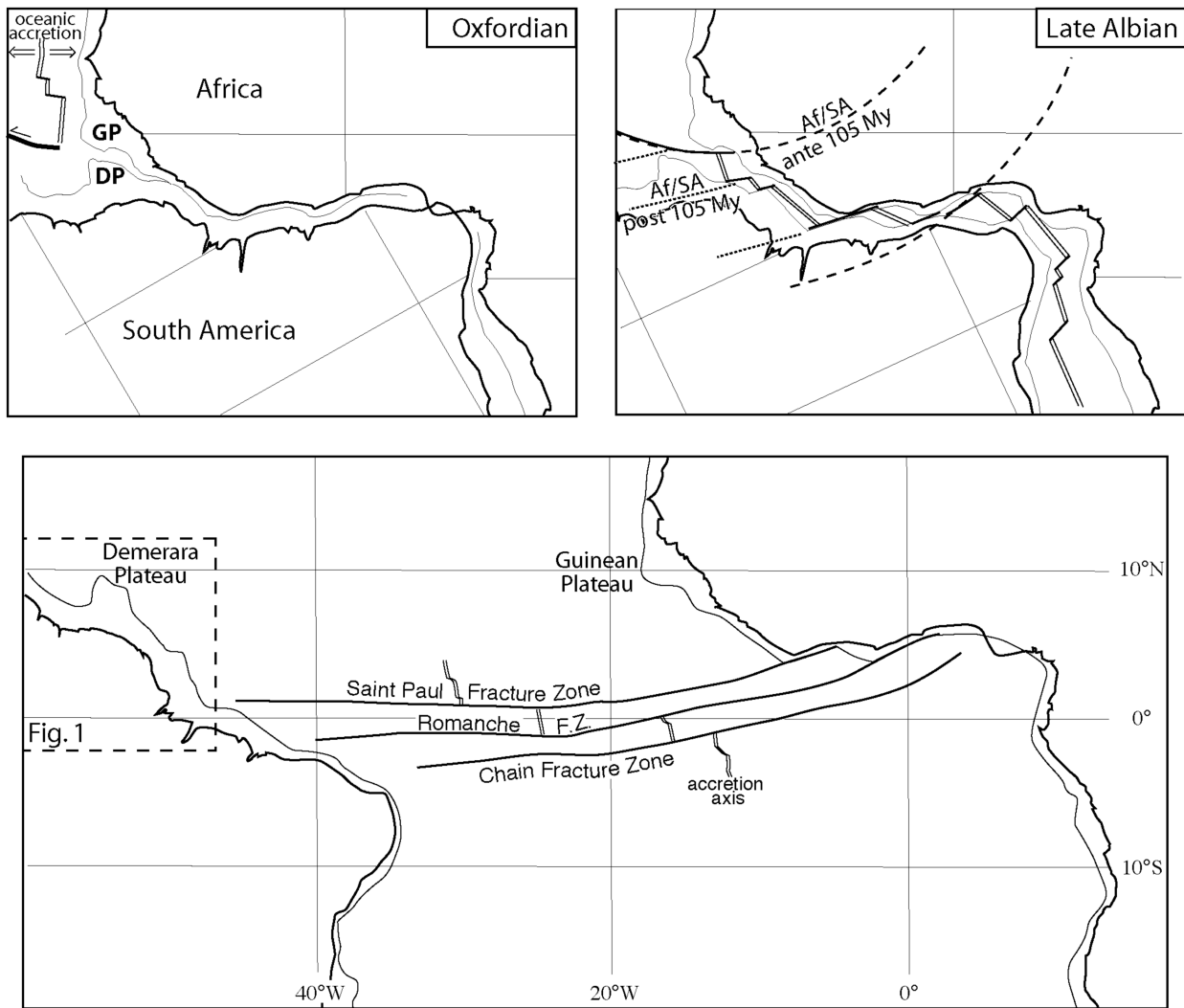
Figure 2 : Present day and reconstructions of Africa – South America positions before (Oxfordian : oceanic spreading in the Central Atlantic) and after the rifting in the Equatorial Atlantic (Late Albian (105 Ma) : oceanic spreading in the South and Equatorial Atlantic). Africa is supposed fixed. The present day coastline and 2 km isobath are drawn. DP and GP are Demerara plateau and Guinea plateau, respectively. The dotted curves in the Late Albian reconstruction are the small circles parallel to the relative motion of South America by reference to Africa, and show the plate kinematic reorganization occurring at 105 Ma. Modified from Basile et al. (2005) and Campan (1995).
