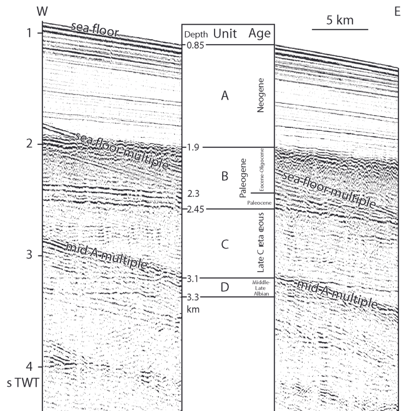
Figure 3 : Seismic units (A to D) from seismic line GUYAPLAC 63, and stratigraphy and approximate depths from well G2 (Gouyet, 1988). The seismic line is located in Figures 1 and 5. Depth in second double way (sdw). Vertical exaggeration 13 in water.
