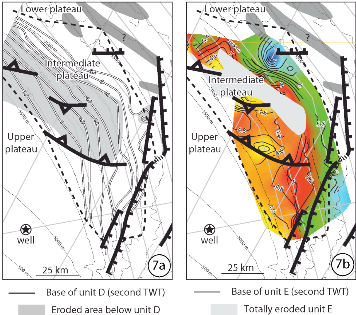
Figure 7 : Depths of the base of unit D (7a) and E (7b) in the intermediate plateau. Structures and bathymetry as in Figure 5. Due to limited seismic penetration, the base of unit E can not be observed in the deepest parts, and the color interpolation is only weakly constrained.
