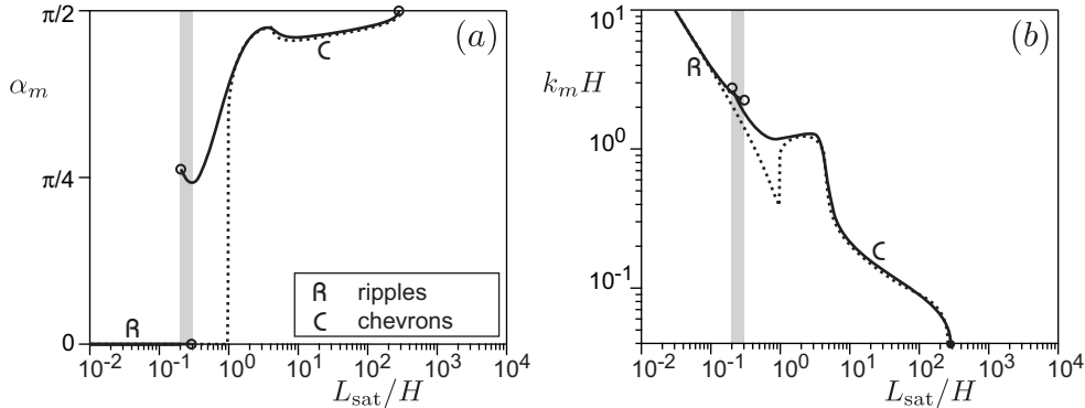
FIGURE 13. Wavelength k_m and angle \alpha_m of the most unstable mode as a function of L_{sat}/H , in the limit u_* / u_{th} \rightarrow \infty . The solid line corresponds to \mathcal{F} = 0.8 (transitions at L_{sat}/H \simeq 0.2 , at \simeq 0.3 and at \simeq 2.9 \cdot 10^2 marked by \circ ) and the dotted line to the limit \mathcal{F} \rightarrow 0 (solid line in Fig. 7). The gray zone indicates the simultaneous existence of two growth rate maxima of comparable amplitude.
