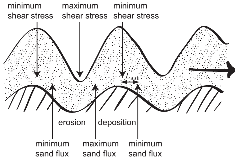
FIGURE 14. Schematic view of anti-dunes and sketch of the instability mechanism. The saturation length L_{sat} represents the spatial lag between the shear stress and the sediment flux.
