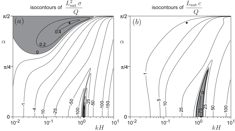
FIGURE 17. (a) Growth rate \sigma as a function of the rescaled wavenumber kH and of the angle \alpha for L_{\text{sat}}/H = 5 , \mathcal{F} = 1 and H/z_0 = 10^2 in the limit u_* / u_{\text{th}} \rightarrow 1 . Isocontours for L_{\text{sat}}^2 \sigma / Q = -150, -100, -50, -25, -10, -4, -1, 0, -0.2, 0.2, 0.4, 0.421, 1.5 . Two local maxima can be observed (●). (b) Propagation speed c in the same conditions. Isocontours for L_{\text{sat}} c / Q = -75, 0, 1, 5, 10, 25, 50, 100
