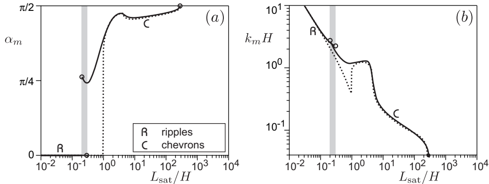
FIGURE 13. Wavelength k_m and angle \alpha_m of the most unstable mode as a function of L_{\text{sat}}/H , in the limit u_* / u_{\text{th}} \rightarrow \infty . The solid line corresponds to \mathcal{F} = 0.8 (transitions at L_{\text{sat}}/H \simeq 0.2 , at \simeq 0.3 and at \simeq 2.9 \cdot 10^2 marked by \circ ) and the dotted line to the limit \mathcal{F} \rightarrow 0 (solid line in Fig. 7). The gray zone indicates the simultaneous existence of two growth rate maxima of comparable amplitude.
