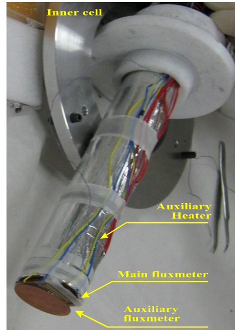
Figure 1b: Implementing heat flow meters
