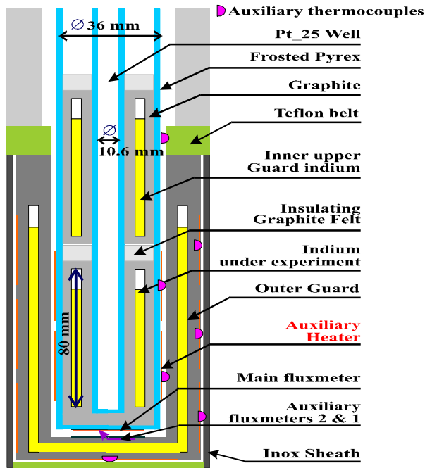
Figure 1a: Cell-within-cell configuration
