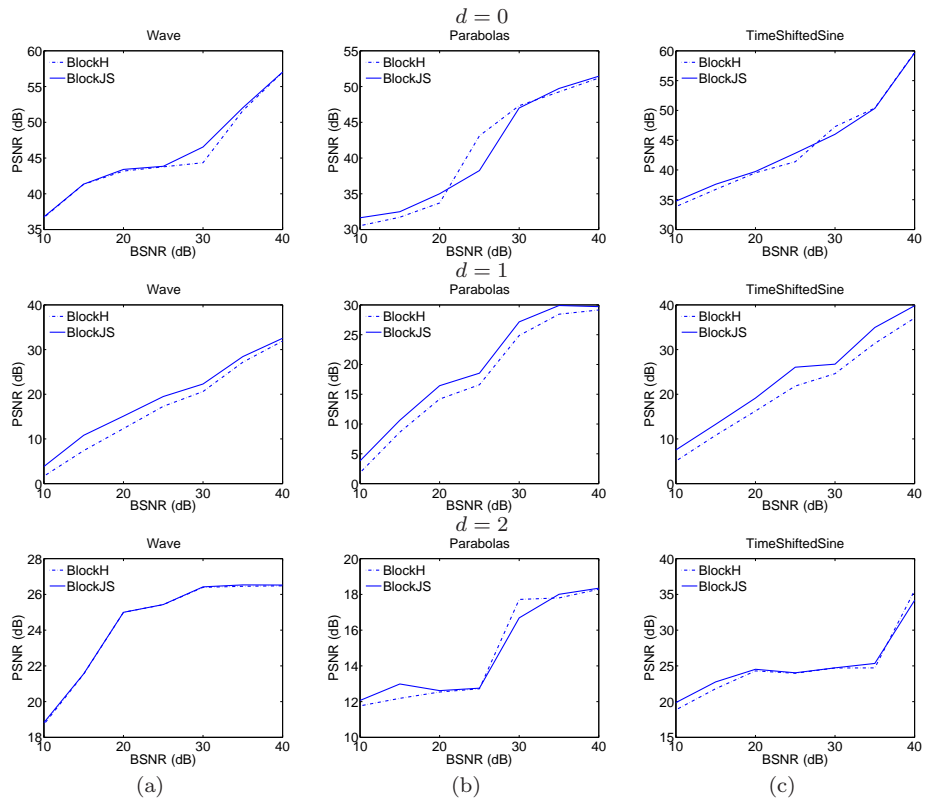
FIG 3. PSNR values as a function of the initial BSNR from 10 replications for (a): Wave. (b): Parabolos. (c): TimeShiftedSine from top to bottom d = 0, 1, 2 .
