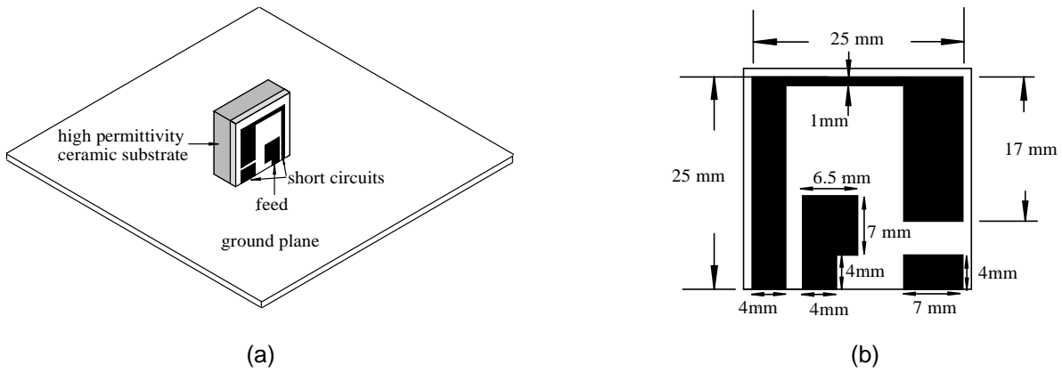
Figure 2 : Overview of the narrow band antenna represented by the association of a printed antenna and a ceramic substrate (a) and a zoom of the radiating element with its main dimensions (b).
