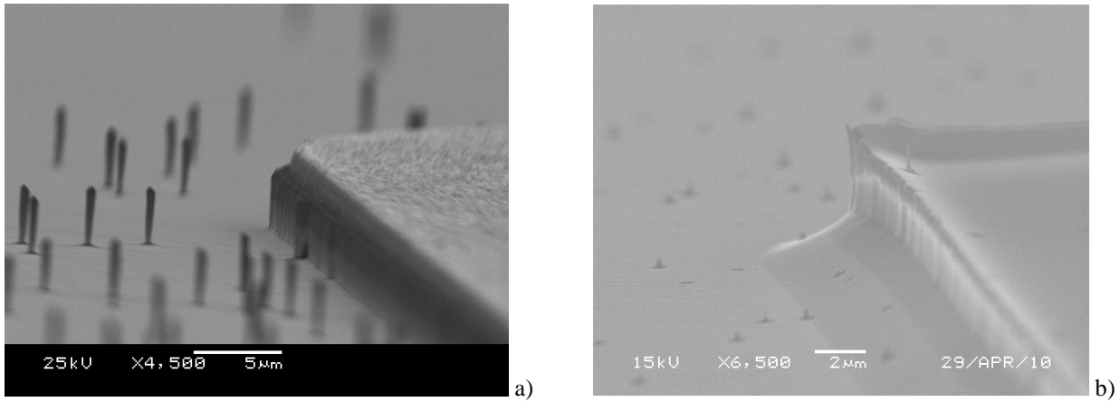
Fig. 1. Examples of micromasking artifacts produced by deposited particles extracted from the mask close to an etched trench (a) and from the cathode electrode made in Al (b).
