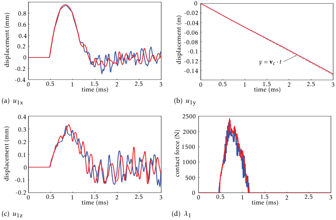
Figure 6: Frictionless low speed configuration; proposed algorithm (—) and bi-potential method (—)
