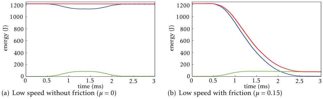
Figure 12: Total (—), kinetic (—), and strain (—) energies versus time
