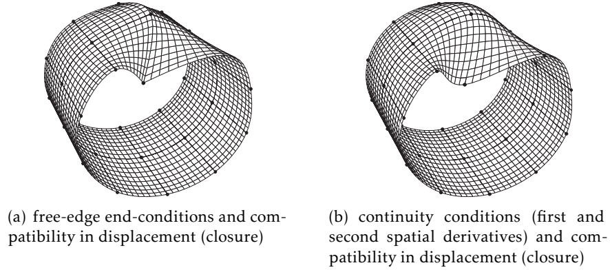
Figure 3: Surface spline versus end-conditions along the circumferential direction. Free-edge end-conditions in the axial direction. Black dots • are the data points of the deformed casing. The control points and vertices are not shown.
