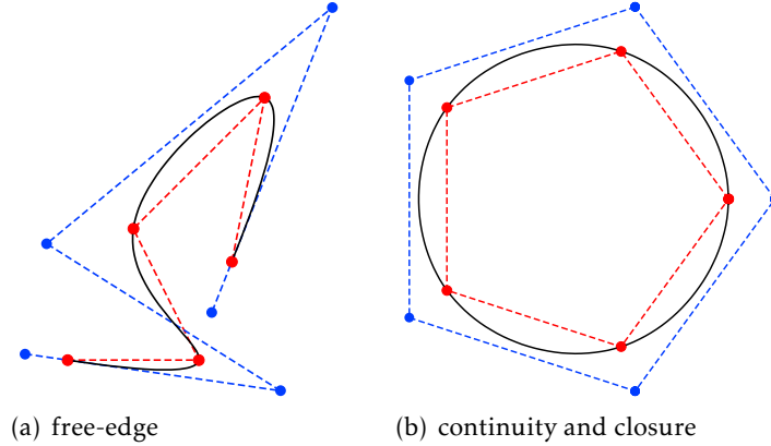
Figure 2: two types of end condition: spline (—), data points P (•) and control points Q (•)
