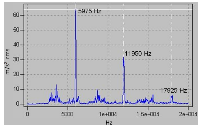
Fig. 21 Test with Vibroport 41; V_c=80 m/min; f=0.125 mm/rev
