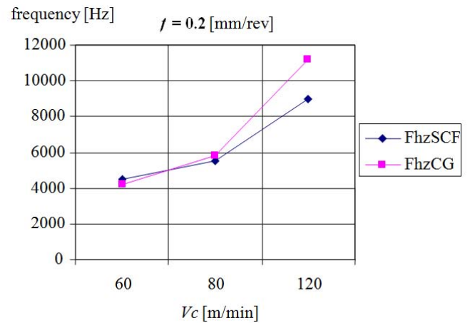
Fig. 20 Frequency accompanying saw-tooth chip formation depending on cutting speed f = 0.2 (mm/rev)
