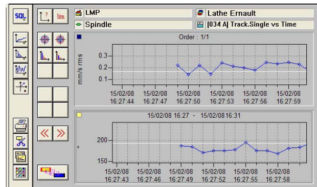
Fig. 4 Vibration level of the Ernauld lathe using Tracking versus time procedure.
