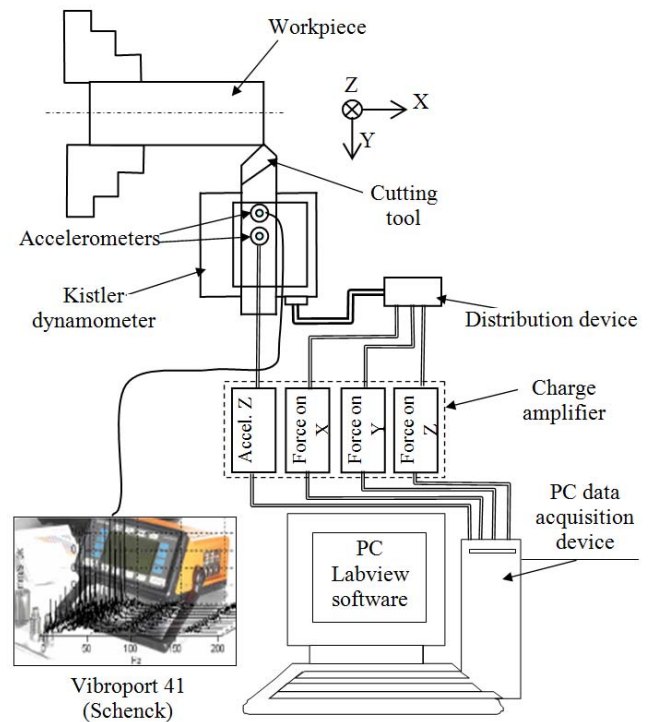
Fig. 18 Experimental acquisition chain in turning process
