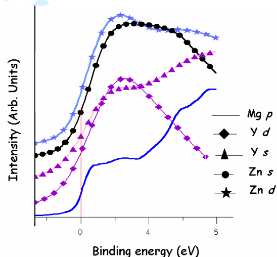
Fig. 2-d: Conduction band of hexagonal \text{Mg}_{28}\text{Zn}_{65}\text{Y}_7 . For clarity, the spectral curves are shifted along the y-axis.
