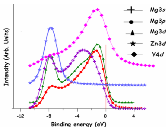
Fig. 2-c: Valence band of hexagonal \text{Mg}_{28}\text{Zn}_{65}\text{Y}_7 . For clarity, the curves are shifted along the y-axis.
