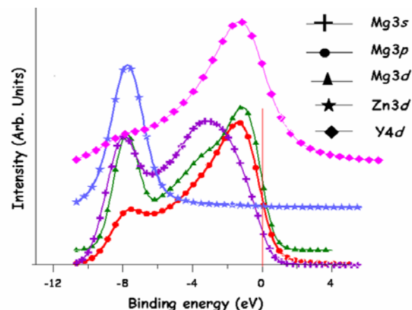
Fig. 2-c: Valence band of hexagonal \text{Mg}_{28}\text{Zn}_{65}\text{Y}_7 . For clarity, the curves are shifted along the y-axis.
