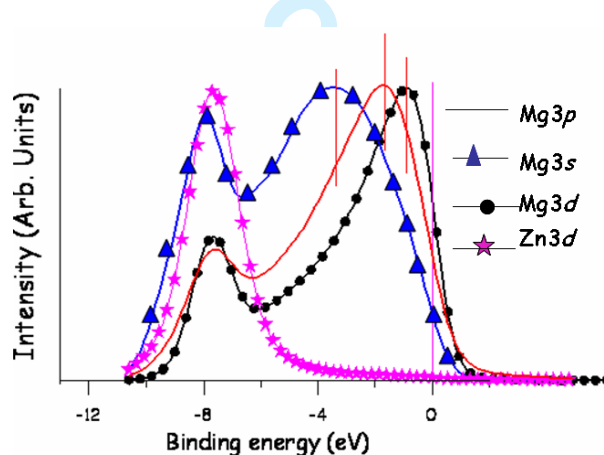
Fig. 2-a: Valence band of \text{MgZn}_2 . The respective maxima are shown by vertical bars.
