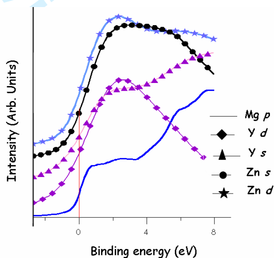
Fig. 2-d: Conduction band of hexagonal \text{Mg}_{28}\text{Zn}_{65}\text{Y}_7 . For clarity, the spectral curves are shifted along the y-axis.
