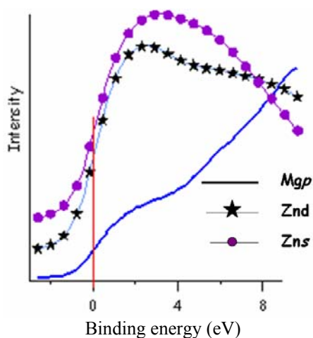
Fig. 2-b: Conduction band of \text{MgZn}_2 . For clarity, the spectral curves are shifted along the y-axis.
