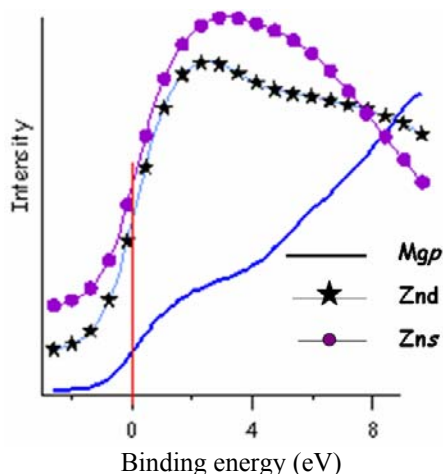
Fig. 2-b: Conduction band of \text{MgZn}_2 . For clarity, the spectral curves are shifted along the y-axis.
