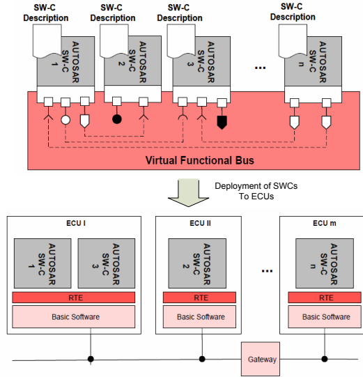
Fig. 2. AUTOSAR methodology
