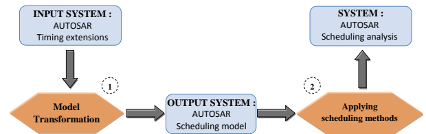
Fig. 1. AUTOSAR model transformation
