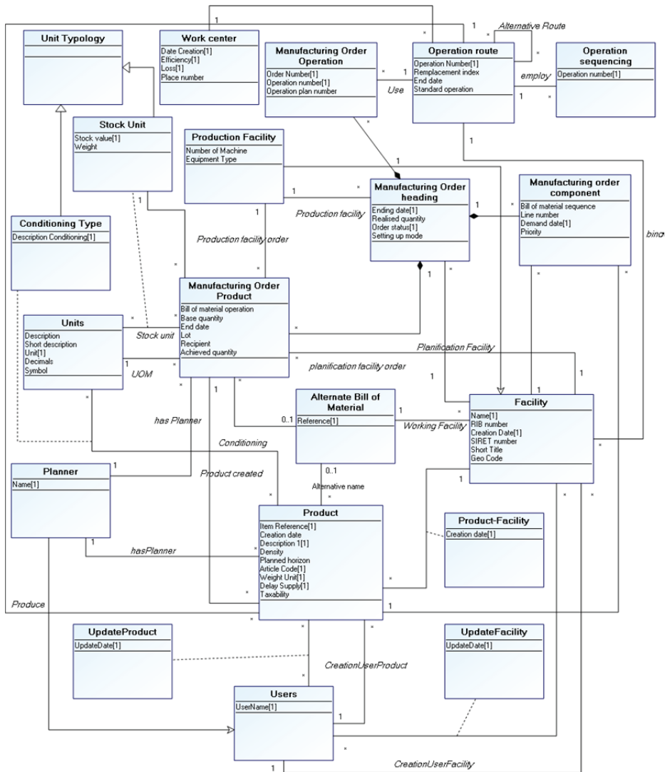
Figure 2 - Sage X3 work order enriched process model
