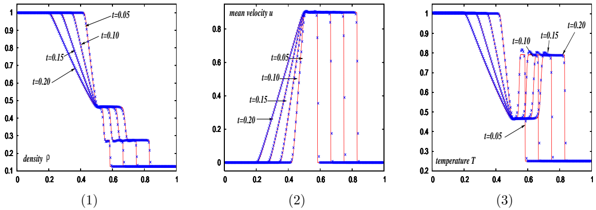
FIGURE 7. Riemann problem ( \varepsilon = 10^{-8} ), comparison with the solution to the Euler system: evolution of (1) the density \rho , (2) mean velocity u , and (3) temperature T at time t = 0.05, 0.1, 0.15 and 0.2 .
