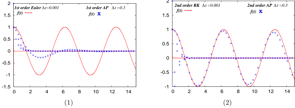
FIGURE 1. Comparison of the time evolution of the numerical approximation to the differential system (2.9)-(2.10) with f(0) = (2, 1, 1) . (1) first and (2) second order Asymptotic Preserving and explicit Runge-Kutta schemes
