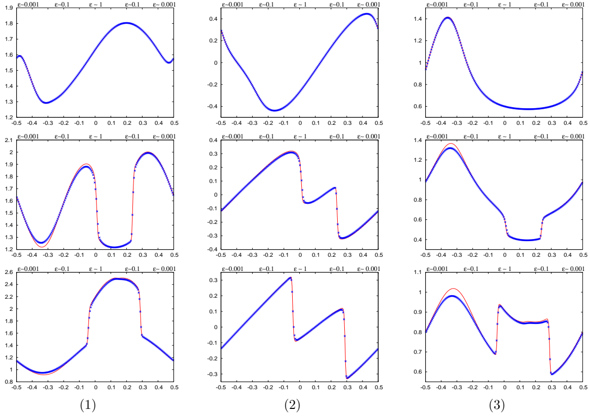
FIGURE 8. Mixing regime problem ( \varepsilon_0 = 10^{-3} ), comparison of the numerical solution to the Boltzmann equation with the second order method (4.14) represented with crosses (x) with the numerical solution obtained with the explicit Runge-Kutta method using a small time step (line): evolution of (1) the density \rho , (2) mean velocity u , (3) temperature T at time t = 0.25, 0.5 and 0.75 .
