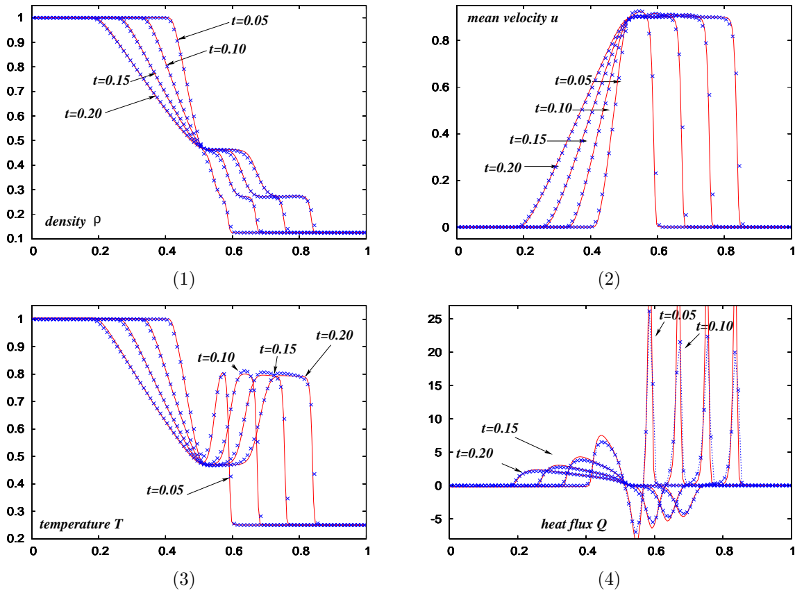
FIGURE 5. Riemann problem ( \varepsilon = 10^{-3} ), crosses (x) represent the numerical solution obtained with our second order method (4.14) and lines with the explicit Runge-Kutta method: evolution of (1) the density \rho , (2) mean velocity u , (3) temperature T and (4) heat flux Q at time t = 0.05, 0.1, 0.15 and 0.2 .
