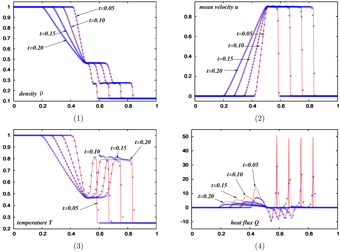
FIGURE 6. Riemann problem ( \varepsilon = 10^{-4} ), comparison between the numerical solution to the Boltzmann equation with our second order method (4.14) represented with crosses (x) and the numerical solution to the compressible Navier-Stokes system (lines): evolution of (1) the density \rho , (2) mean velocity u , (3) temperature T and (4) heat flux Q at time t = 0.05, 0.1, 0.15 and 0.2 .
