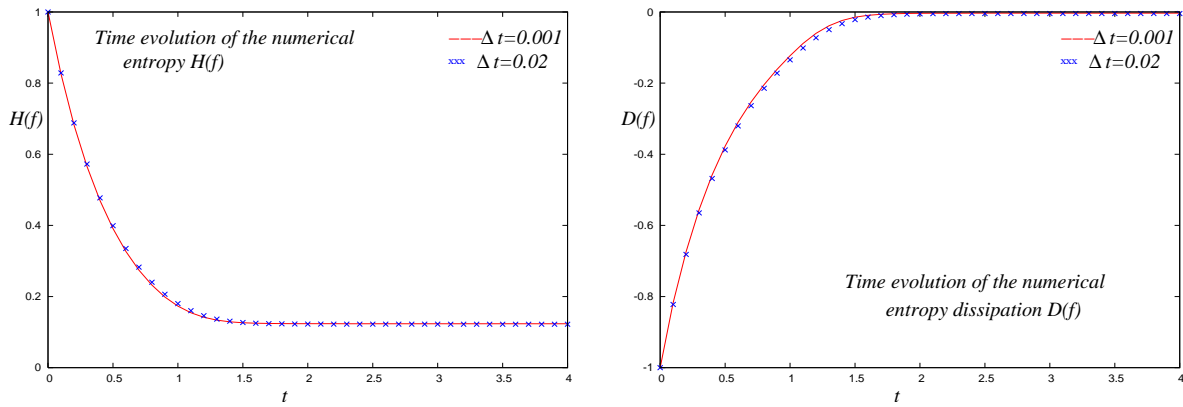
FIGURE 11. Nonlinear Fokker-Planck solution: convergence toward equilibrium (Barenblatt-Pattle distribution) obtained with the first order method (2.6) using n_x = 100 with \Delta t = 0.02 and 0.001 .
