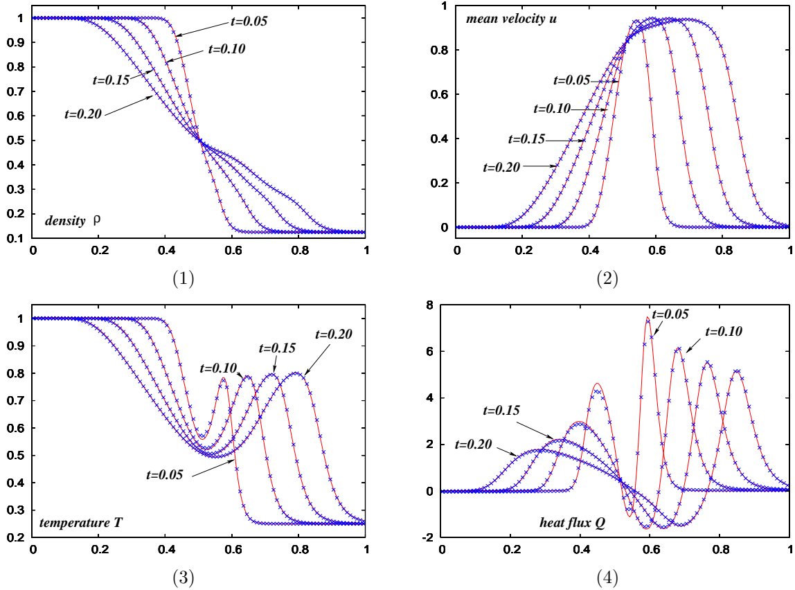
FIGURE 4. Riemann problem ( \varepsilon = 10^{-2} ), crosses (x) represent the numerical solution obtained with our second order method (4.14) and lines with the explicit Runge-Kutta method: evolution of (1) the density \rho , (2) mean velocity u , (3) temperature T and (4) heat flux Q at time t = 0.05, 0.1, 0.15 and 0.2 .
