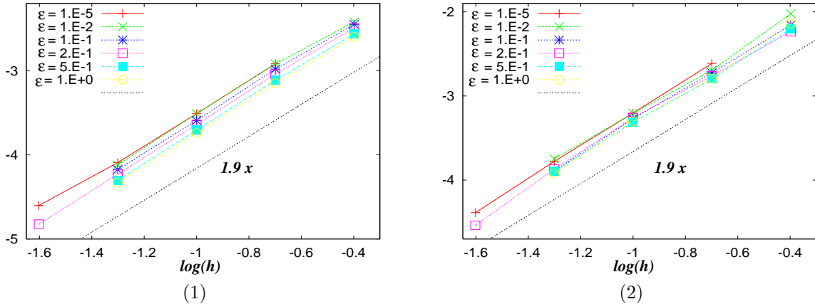
FIGURE 3. The L^1 and L^\infty errors of the second order method (4.14) for different values of the Knudsen number \varepsilon = 10^{-5}, \dots, 1 .
