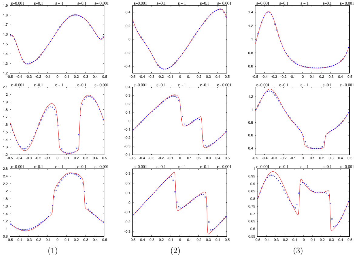
FIGURE 9. Mixing regime problem ( \varepsilon_0 = 10^{-3} ), comparison of the numerical solution to the Boltzmann equation obtained with the AP scheme (4.14) using n_x = 50 (crosses \mathbf{x} ) and n_x = 200 points (line): evolution of (1) the density \rho , (2) mean velocity u , (3) temperature T at time t = 0.25, 0.5 and 0.75 .
