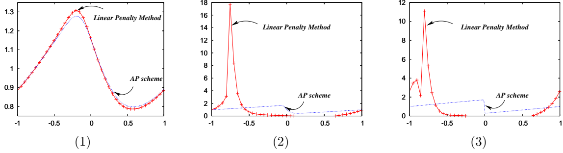
FIGURE 2. Approximation of the solution to (3.8) obtained from our AP scheme (3.1) and the linear penalty method (3.4) for different values of the Knudsen number \varepsilon = 10^{-1}, 10^{-2} and 10^{-7} .
