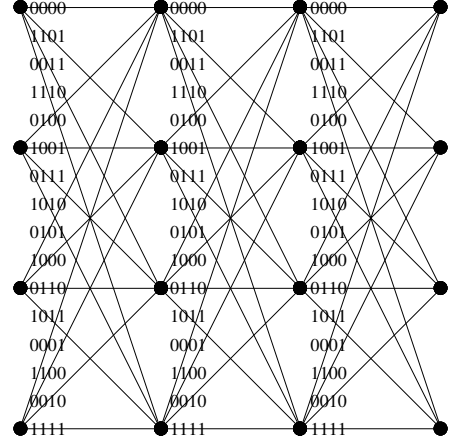
Fig. 3. 4-state trellis of the convolutional Hamming code.
