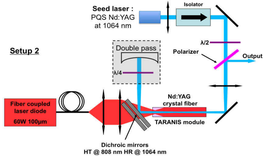
Fig.5 Experimental setup 2: this first pass is in counter-propagation, the second pass is in co-propagation. In this section, the seed laser emitted 1 ns pulses at 100 kHz with an average power of 350 mW. It will be replaced by other seed lasers in the sections 4 and 5.
