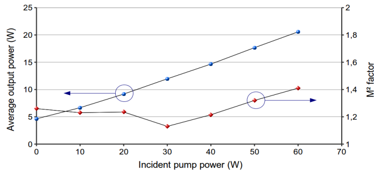
Fig. 8. Output average power (blue circle) and M^2 factor (red square) versus the incident pump power with the PicoSpark™ in a simple pass configuration.
