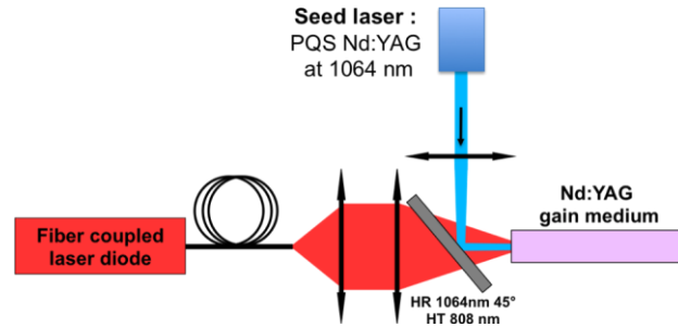
Fig.1. Experimental setup for the test of the amplifiers.
