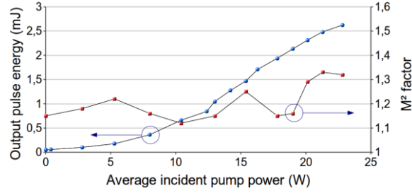
Fig.11. Output energy in double pass configuration versus the pump power (left). M^2 factor versus the pump power (right).
