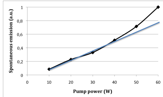
Fig.7. Spontaneous emission collected from the pump face versus the pump power.
