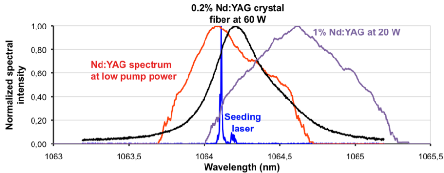
Fig.3. Normalized fluorescence spectrum recorded at different pump powers for 0.2% doped Nd:YAG crystal fiber and for 1% doped Nd:YAG. The spectrum of the seeding laser is also added on the graph. The spectra at low pump power and for the 1% Nd:YAG are more noisy than the spectrum of the 0.2% Nd crystal fiber because the amount of spontaneous emission was much lower.
