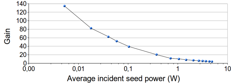
Fig. 9. Gain versus the average incident signal power with the PicoSpark™ laser source in a simple pass configuration for 60 W of incident pump power.
