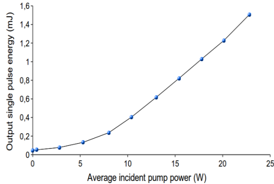
Fig.10. Output energy in single pass configuration versus the pump power.
