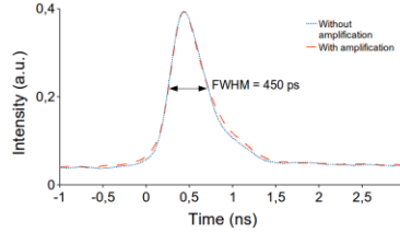
Fig.12. Duration of the output pulses after two pass amplification and without amplification (recorded with a 4GHz single shot oscilloscope).
