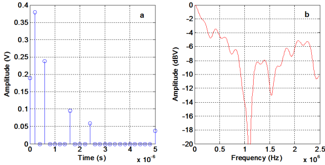
Figure 1. Example of a CIR in the delay (a) and frequency (b) domains
