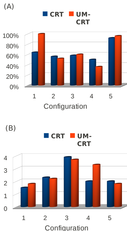
Figure 5 : Received packets rate (A) and mean number of hops (B) in the MIMO case
