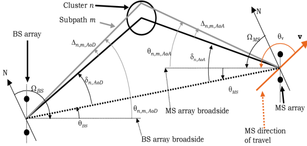
Figure 1 : Angular parameters of the SCME model
