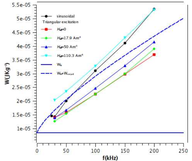
Fig. 2. Total losses measured under sinusoidal excitation (full circular black points), triangular unbiased (full red square points), triangular biased with offset field H_{off} = 17.9 \text{ Am}^{-1} (full diamond green point), 50 \text{ Am}^{-1} (upward full triangle), 110.3 \text{ Am}^{-1} (downward full triangle). The dashed line represents the sum of the hysteresis losses W_h and the spin dumping excess losses W_{exc,sd} calculated using expression (5) with n = 0.3 , \alpha_{LL} = 0.06 and k_{irr} = 0.18 . The full line represents the hysteresis losses extrapolated from the measurements
