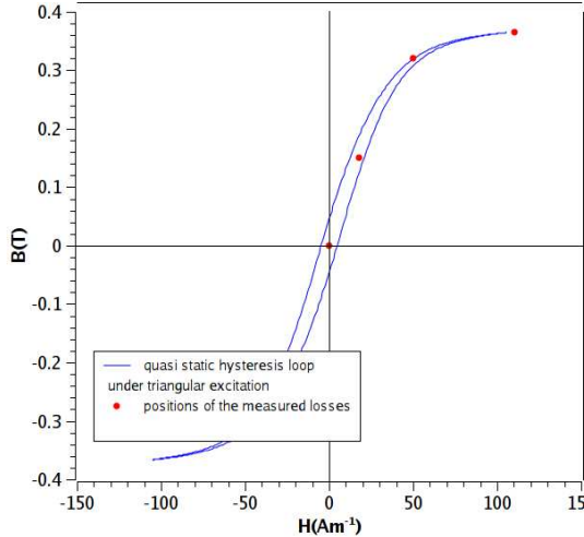
Fig. 1. Quasistatic hysteresis loop measured with fluxmetric method. The points represent the position where losses have been measured. Starting from the demagnetised state the points correspond respectively to the following bias field: H_{off} = 0, 17.9, 50, 110.3 \text{ Am}^{-1}
