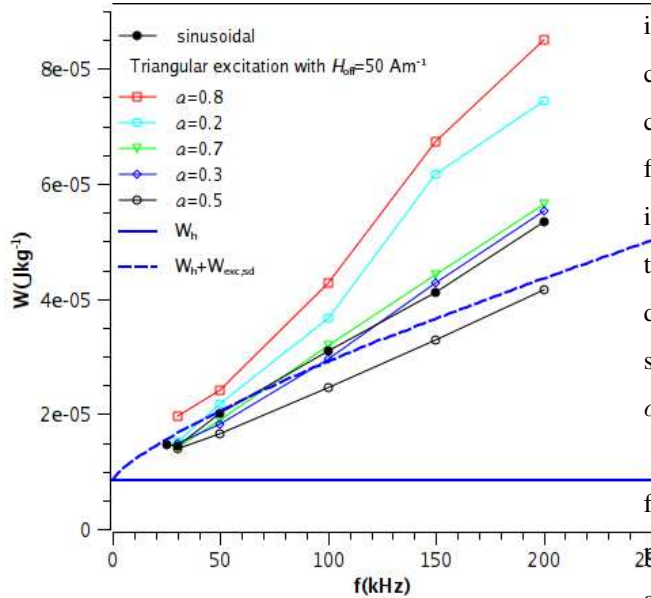
Fig. 3. Total losses measured under sinusoidal excitation (full circular black points), triangular biased ( H_{off} = 50 \text{ Am}^{-1} ), with different degrees of asymmetry. The lines represents the same curves plotted in Fig. 2
