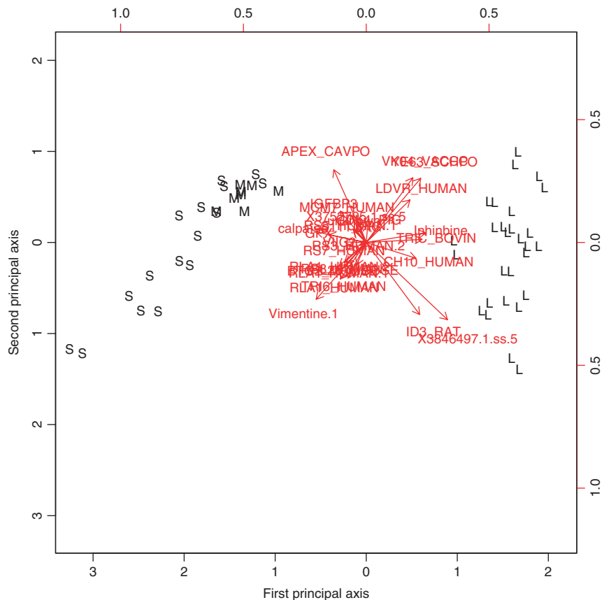
Figure 2 Biplot of the principal component analysis performed on the top-29 differentially expressed genes. The first two principal axes explain 68% and 8% of the total variability.
