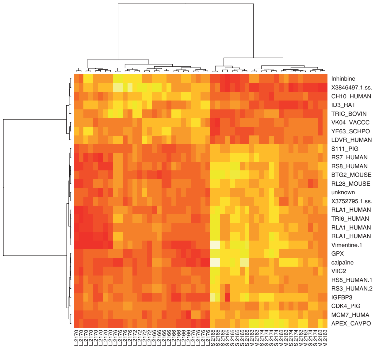
Figure 3 Heat map display of unsupervised hierarchical clustering results (Ward method and Euclidian distance) of the top-29 most significant genes. Genes are displayed in lines and membranes in columns. The light (respectively, dark) colour represents up- (respectively, down-) regulated genes.
