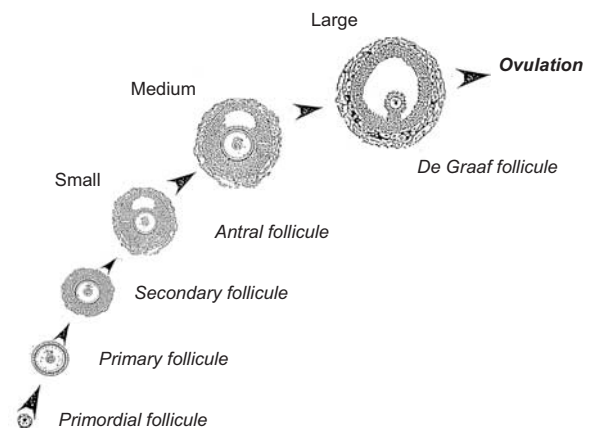
Figure 1 Scheme of folliculogenesis. Follicles grow from a primordial type to De Graaf type prior to ovulation. The follicles of the current analysis (small, medium-sized and large) correspond to Antral and De Graaf types.
