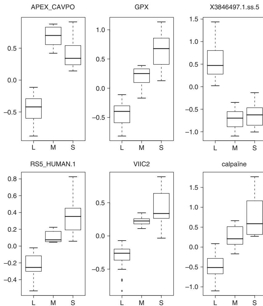
Figure 4 Boxplots of some of the most discriminant (or predictive) genes from the random forest analysis, also in the top-29 list.
