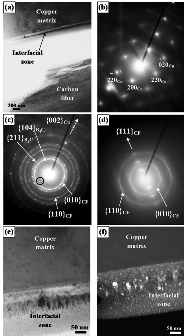
Fig. 6. TEM analyses of sample S9. (a) Bright field of the zone with, from top to bottom, the Cu matrix, the interface and the CF; (b) diffraction pattern of the Cu matrix [001] copper axis); (c) diffraction pattern of the interfacial zone; (d) diffraction pattern of the CF; (e) zoom on the interfacial zone and (f) dark field of the interfacial zone using the \{104\} B_4C diffraction ring marked on (c).
