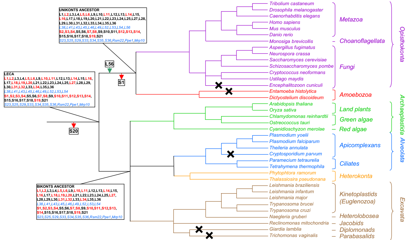
Fig. 2. Inference of the set of MRPs present in the last eukaryotic common ancestor and its subsequent evolution in Unikonts and Bikonts. MRP acquisitions are indicated by green arrows, whereas losses are highlighted by red arrows. Proteins of alphaproteobacterial origin encoded in mitochondria are indicated in bold. Bt-MRPs predicted to be encoded in mitochondria are indicated in red, whereas those encoded in the nucleus are indicated in black. EK-MRPs are indicated in blue italic font. Lineages that have lost their mitochondria are marked with crosses; in these cases no ribosomal proteins are detected in their genomes, to the exception of Ppe1 (but see text for discussion).
