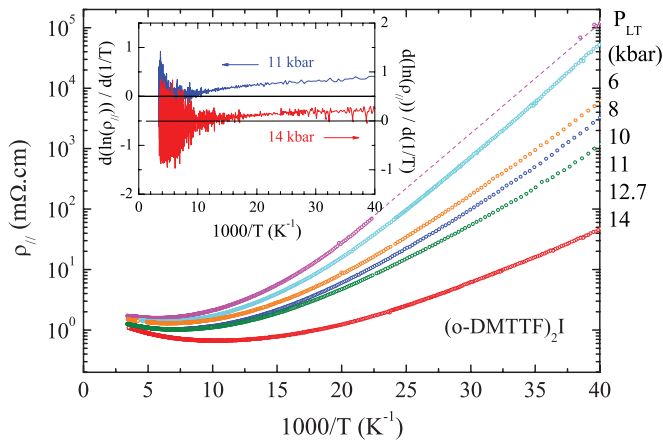
FIG. 6. (Color online) Evolution of the longitudinal resistivity versus the inverse of the temperature for different pressures in (o\text{-DMTTF})_2\text{I} . Insert: d(\ln(\rho))/d(1/T) as a function of temperature at 11 and 14 kbar showing the absence of any clear maximum around 50 K.
