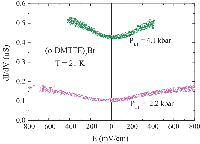
FIG. 5. (Color online) Longitudinal differential conductance versus the applied electric field in (o\text{-DMTTF})_2\text{Br} at 21 K for the two pressures shown in Fig. 4(a).
