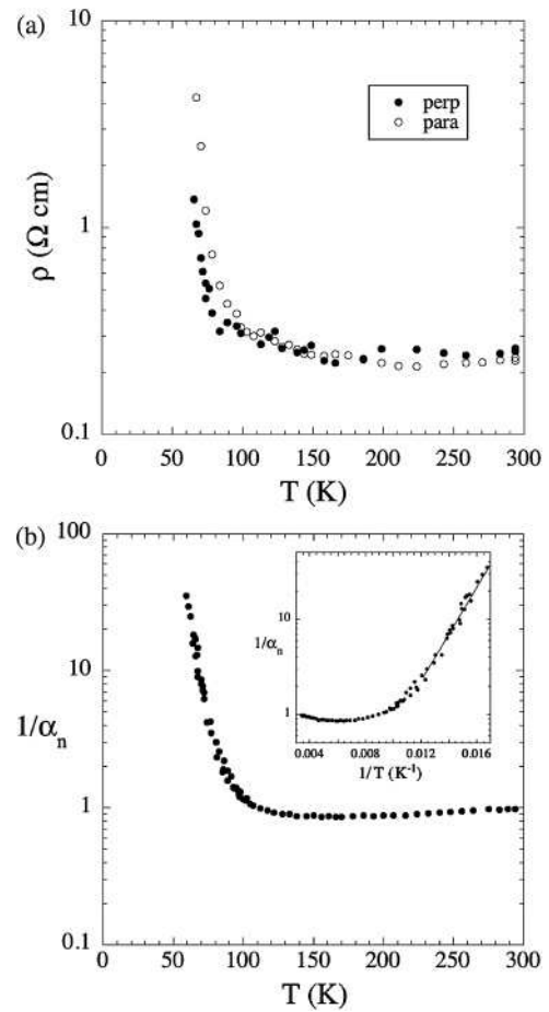
FIG. 12. (a) Temperature dependence of the transverse resistivity deduced from ESR data along the two principal magnetic directions for (o\text{-DMTTF})_2\text{Br} at ambient pressure. (b) Temperature dependence of 1/\alpha normalized at room temperature, deduced from ESR data for (o\text{-DMTTF})_2\text{Cl} at ambient pressure. In the inset, the same data plotted as a function of 1/T demonstrates the activated regime below 80 K.
