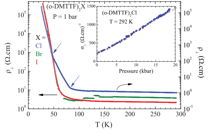
FIG. 2. (Color online) Transverse resistivity as a function of temperature for the (o-DMTTF) 2 X series at ambient pressure. Inset: evolution of the room-temperature longitudinal conductivity with pressure in (o-DMTTF) 2 Cl.
