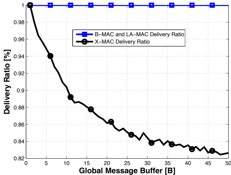
Figure 24: Delivery ratio vs. the global message buffer. In X-MAC, most collisions happen when messages are sent after the back-off time.
