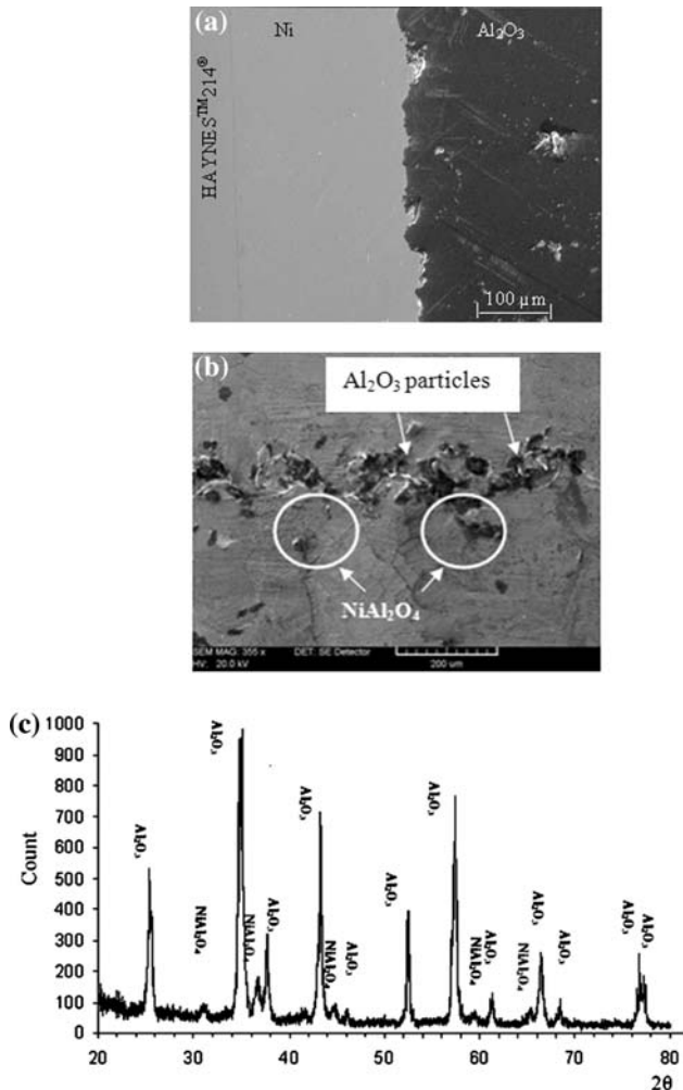
Fig. 6 a Cross section of Al 2 O 3 /Ni interface formed by diffusion bonding, b SEM micrograph of sample diffusion bonded at 1150 °C for 60 min, showing the top of Ni after fracture of Al 2 O 3 /Ni interface, and c GIXRD diffraction patterns of high purity alumina bonding area ( \lambda_{K\alpha} Cu)
