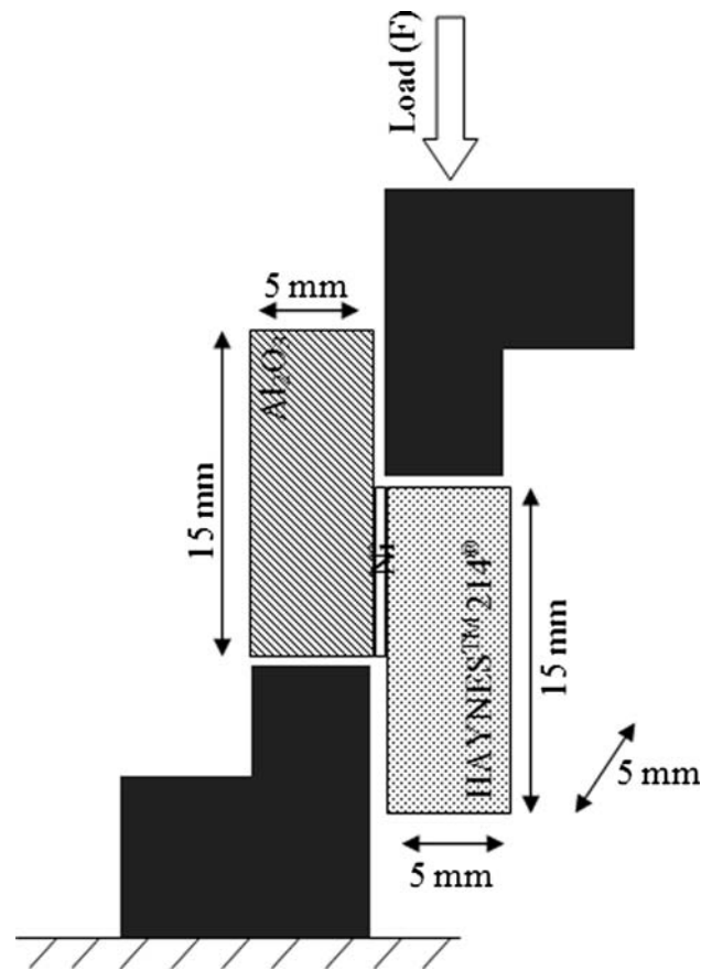
Fig. 2 Mechanical shear test and geometry adapted to the test
