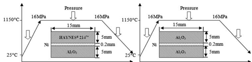
Fig. 1 Sample fabricated for the solid-state bonding, and thermal cycle
