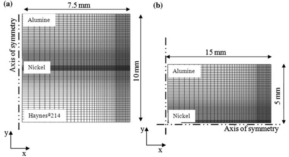
Fig. 3 Schematic representation of the geometry and the mesh configuration used in the FEA simulation. a \text{Al}_2\text{O}_3/\text{Ni}/\text{HAYNES}^{\circledR} 214 and b \text{Al}_2\text{O}_3/\text{Ni}/\text{Al}_2\text{O}_3
