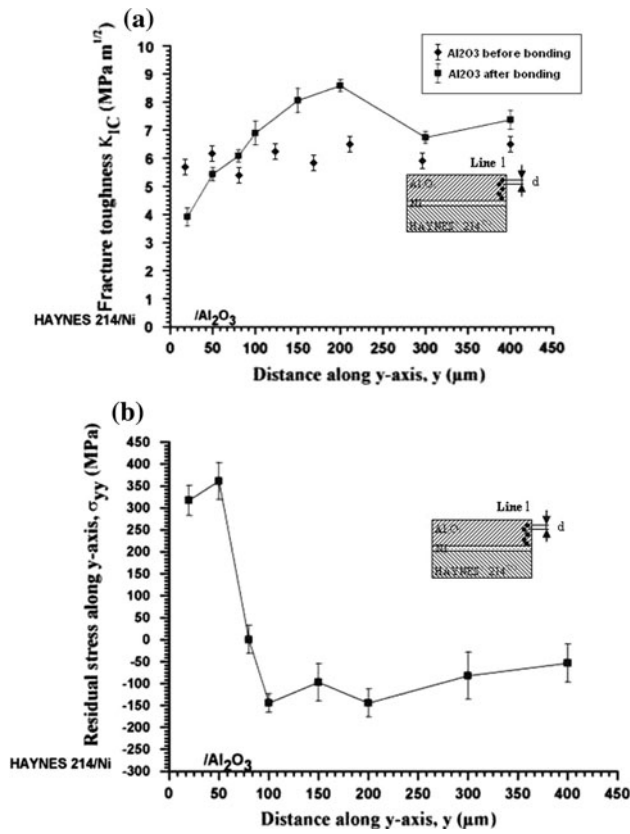
Fig. 5 Evolution of alumina fracture toughness and average residual stress with distance from interface for Al 2 O 3 /Ni/HAYNES ® 214 joint. a Fracture toughness and b residual stress. d is the distance of the Vickers impression
