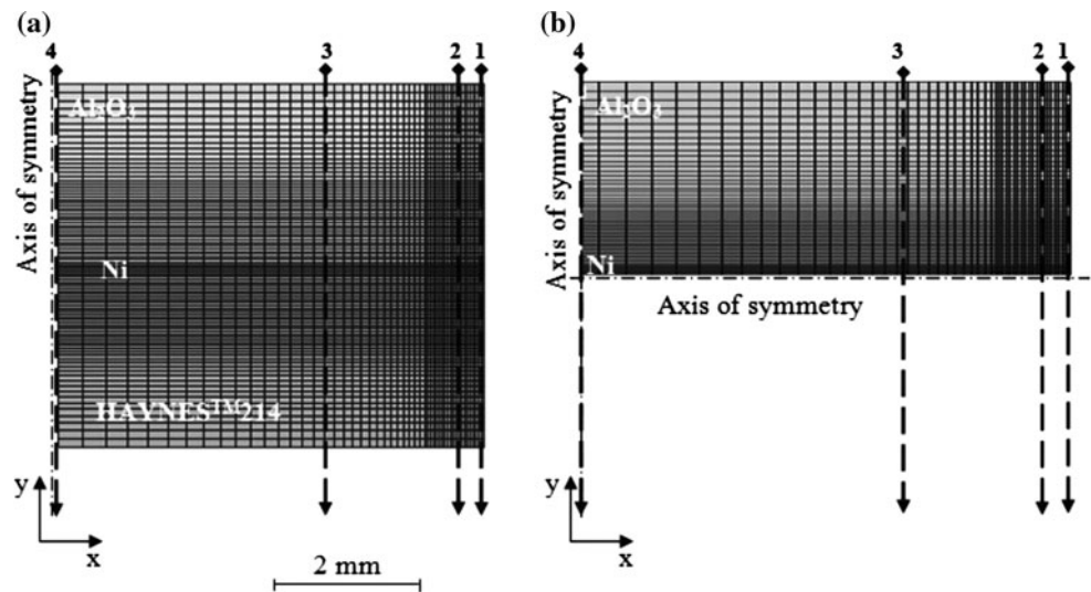
Fig. 2 Geometry of the specimen and the mesh configuration used in the finite-element model. a \text{Al}_2\text{O}_3/\text{Ni}/\text{HAYNES}^{\text{®}} 214^{\text{TM}} joint and b \text{Al}_2\text{O}_3/\text{Ni}/\text{Al}_2\text{O}_3 joint. The numbers 1, 2, 3, and 4 represent the lines where residual stresses variation were plotted
