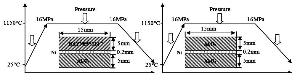
Fig. 1 Schematic drawing of the samples fabricated for the solid-state bonding, and thermal cycle
