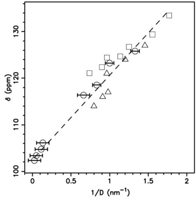
FIG. 3. ^{13}\text{C} NMR isotropic chemical shifts for CNTs versus the inverse of their diameter ( D ): experiments (circles), ab initio calculation (squares) and calculation performed by Sebastiani and Kudin et al. for different tube diameters (triangles). 48 The dashed line corresponds to \delta (see Eq. (1)), the best fit of the experimental data.
