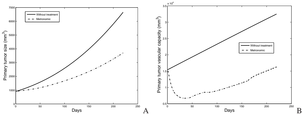
Figure 13: Metronomic schedule for Docetaxel with dose 8 mg/day. A. Tumor size. B. Vascular capacity
