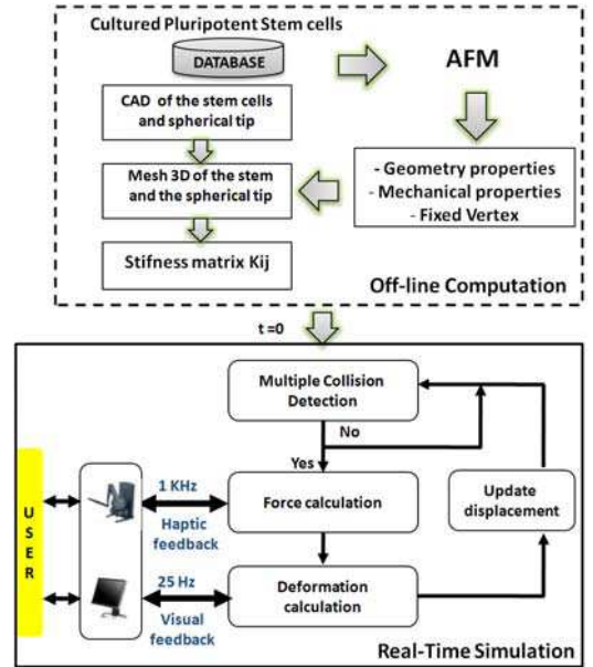
Fig. 2. Computational architecture for simulating force-reflecting deformable cell indentation in virtual environment. The figure shows the two simulation phases used for the real-time indentation of the cell: (i) off-line pre-calculations of stiffness matrices and (ii) simulation of visual and haptic interaction.
