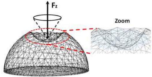
Fig. 11. Depth deformation of the cell; the left picture presents the depth indentation ( 2\mu m ) of the cell, the right picture show the zoom of the cell deformation
