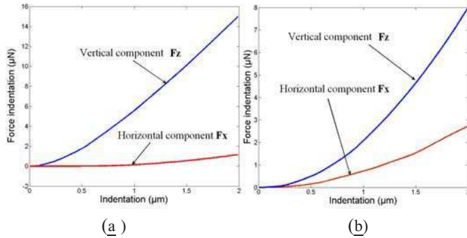
Fig. 13. The horizontal and vertical component force versus indentation, (a); the probe is put in the center of the cell, (b); the probe is put without corresponding to the center of cell.
