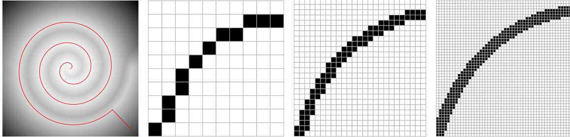
Figure 8: Reference solution for the third test case (left). The Riemannian metric \mathcal{M} is anisotropic only on a thin band along a spiraling curve, wide of a few grid points. Detail at resolutions n \times n , where n equals 200 (center left), 500 (center right) and 1000 (right).
