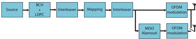
Fig. 2. Block diagram of the transmitter
