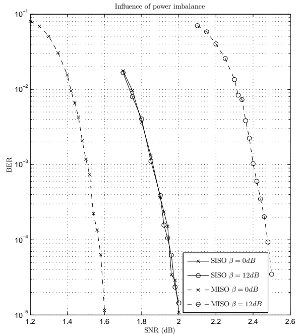
Fig. 5. Influence of power imbalance on the performance of DVB-T2 MISO and SISO transmissions with QPSK and a code rate of 1/2 on TU6 channel
