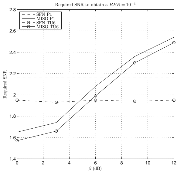
Fig. 6. Required SNR to obtain a BER = 10^{-4} as a function of power imbalance for QPSK and a code rate of 1/2
