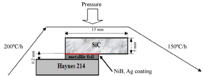
Fig. 1. Schematic view of the sample and of the temperature cycle used for the solid state bonding.
